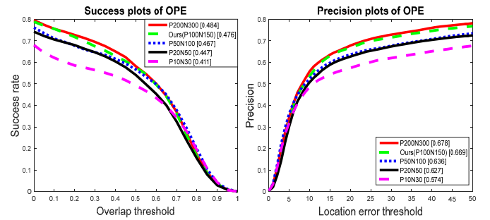
Fig. 9. Success plot and precision plot. The success rate and precision of our proposed tracker under different numbers of positive and negative templates.
