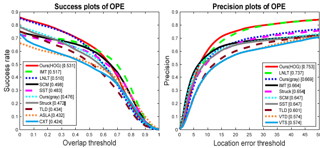
Fig. 4. Success plot and precision plot. The performance score for each tracker is shown in the legend.
