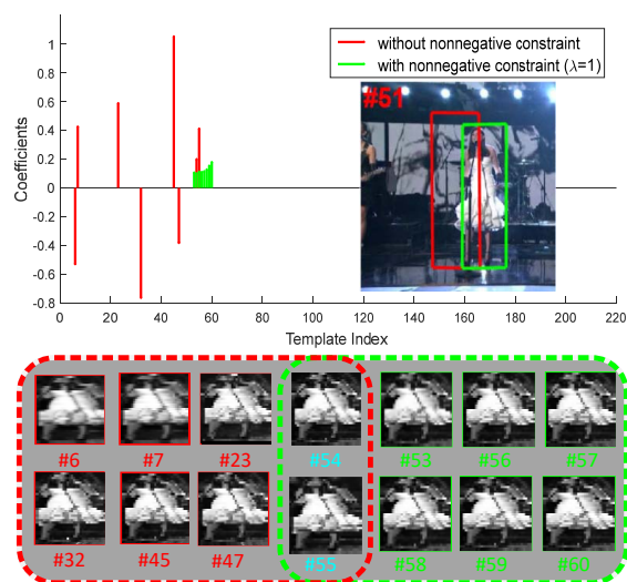
Fig. 1. Illustration of two tracking results in the sequence Singer1 . The good tracking result (in green) is represented by eight positive template images (#53, #54, #55, #56, #57, #58, #59 and #60) with nonnegative coefficients. The bad tracking result (in red) is represented by eight selected positive template images (#6, #7, #23, #32, #45, #47, #54 and #55) with both positive and negative coefficients as illustrated by the figure in the top corner.
