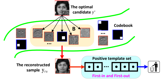
Fig. 3. Template updating scheme for positive template set.
