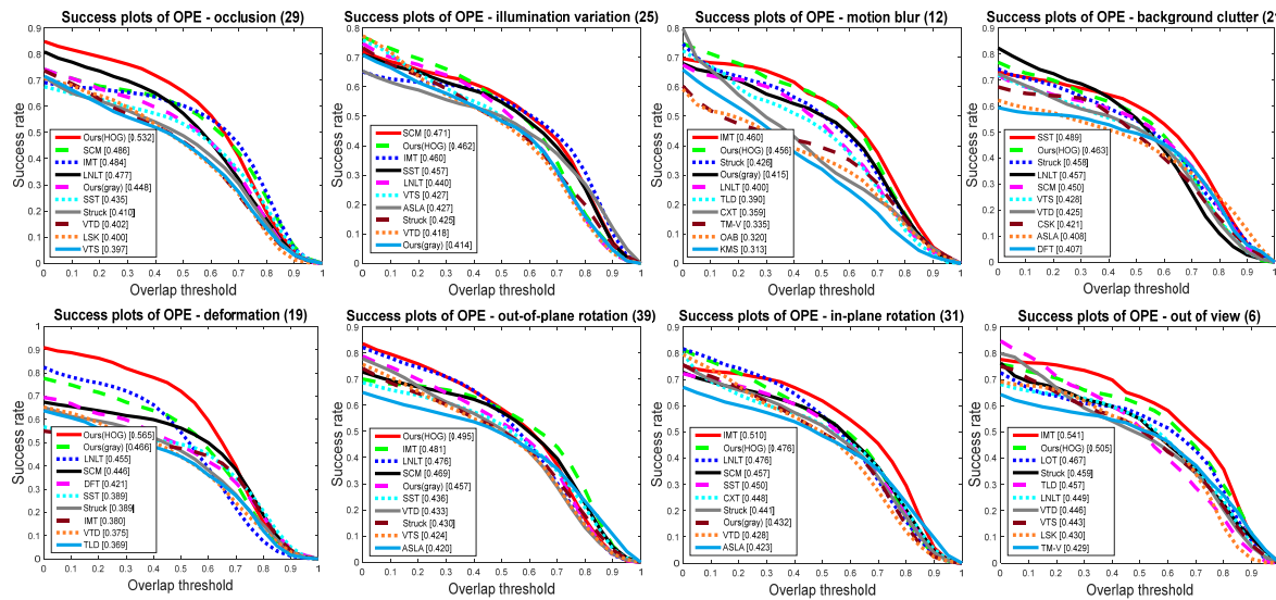
Fig. 5. The curves of success rates of various compared methods on eight main attributes.
