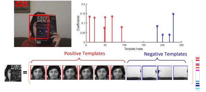
Fig. 2. An occluded target in the sequence FaceOcc1 represented by six positive templates and four negative templates with nonnegative coefficients.
