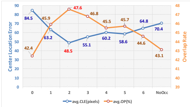
Fig. 8. Tracking performance with varying negative templates threshold. The average CLE and average OP versus the threshold of the number of negative templates (Num(neg * )) are illustrated.
