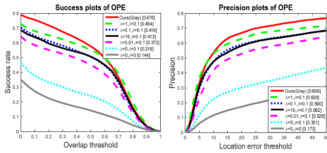
Fig. 7. Success plot and precision plot. The success rate and precision of our proposed tracker under different selections of \lambda and \beta .
