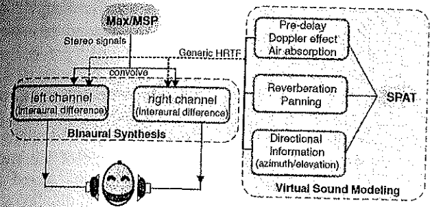
Figure 3: System Overview. The two core units consist of virtual sound modeling and binaural synthesis, which render the virtual realism and realistic sound. Pre-delay (Doppler Effect, air absorption and reverberation) and pre-equalization are accomplished by SPAT. Generic HRTF are used to enhance binaural presentation.
