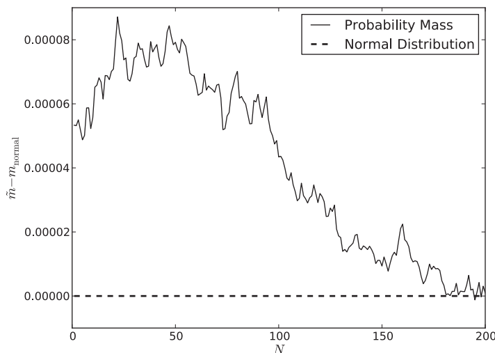
Figure 5. SMC approximated covariance probability mass \tilde{m}(\text{Cov}(\hat{\mathbf{x}})^{-1}/Z^2) for the known- T_2 single-parameter model as compared to the probability mass m_{\text{normal}} \approx 0.9973 expected for the normal distribution and as a function of the number N of experiments performed, averaged over 20 119 trials using a guess heuristic that chooses the k th guess to occur at time (9/8)^k , using 30 guesses, 1000 particles and NCG optimization. The dashed line shows the probability mass for the corresponding normal distribution.
