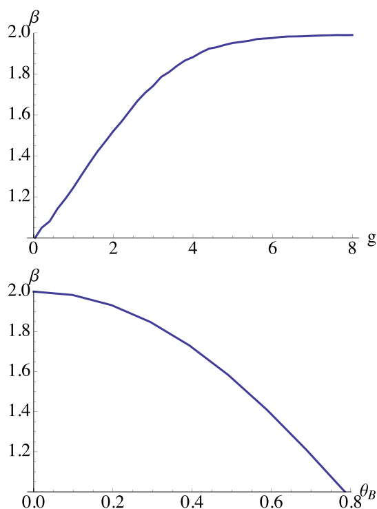
Figure 6 | Exponent of a \sigma^2(t) = t^\beta fit of the variance against time for a self-avoiding walk. \beta = 1 corresponds to linear variance against time, whereas \beta = 2 corresponds to quadratic variance against time (ballistic spread). (top) A classical self-avoiding random walk with self-avoidance function given by Eq. 12, where g is the self-avoidance strength. The fitting is calculated over 200 time steps and 1000 repetitions. When g = 0 we reduce to a normal balanced classical random walk, which exhibits linear spread and thus \beta = 1 (analogous to Fig. 2(e)). As the self-avoidance strength increases, we approach a perfectly self-avoiding random walk, exhibiting maximum quadratic dispersion, and \beta = 2 (analogous to Fig. 2(a)). (bottom) The same fit for a quantum self-avoiding walk where \theta_C = \pi/4 and \theta_M = \pi/2 . This is the classical regime of maximum coupling between the walker and the memory. Now \theta_B takes the role of the self-avoidance strength.
