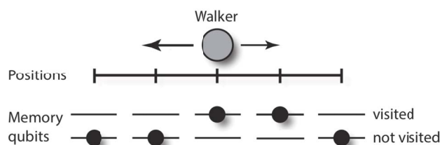
Figure 1 | Illustration of the different subsystems in the self-avoiding quantum walk. The walker resides on a linear graph structure with a two-level memory qubit associated with each vertex, indicating whether the site has been previously visited.
