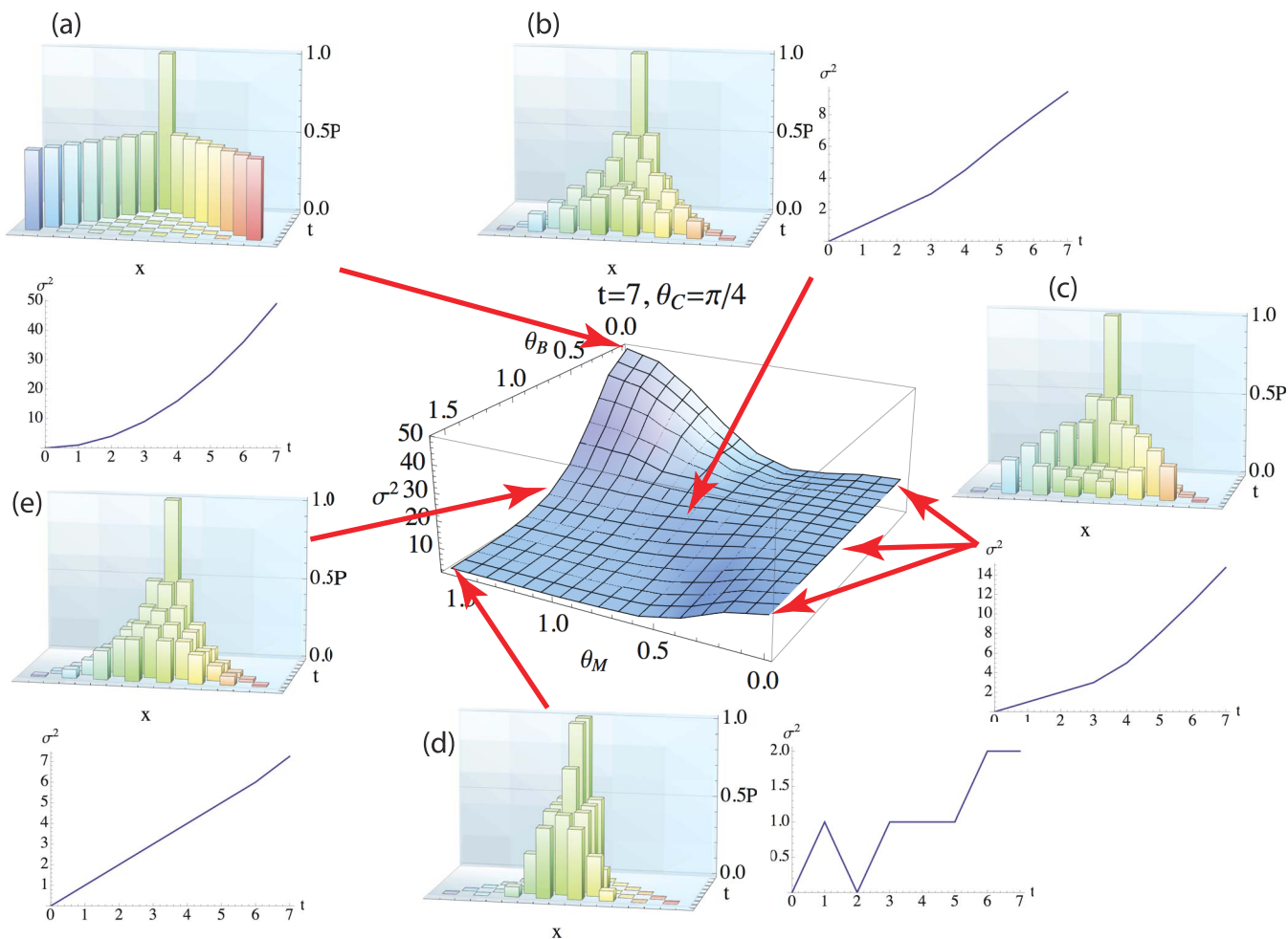
Figure 2 | Final variance ( t = 7 ) of the self-avoiding quantum walk with symmetrised input state (Eq. 8), against memory recording strength ( \theta_M ) and coin back-action strength ( \theta_B ), and, as insets, some of the corresponding quantum walks (showing the full time evolution of the variance and probability distribution). (e) In the limit of \theta_M = \pi/2 and \theta_B = \pi/4 we observe ideal classical random walk statistics, since the memory is maximally entangled with the walker, yielding a balanced \pi/4 walk with decoherence upon tracing out the memory subsystem. (c) In the opposing limit of \theta_M = 0 and irrespective of \theta_B we observe ideal quantum walk statistics, since now the memory does not couple with the walker, yielding a uniform \pi/4 walk without decoherence. The memory never changes, remaining at its initial value. (a) Variance is maximised when \theta_M = \pi/2 and \theta_B = 0 , for which the coin will always be the identity coin, yielding two outward straight line trajectories. (d) When \theta_M = \pi/2 and \theta_B = \pi/2 the dispersion is restricted since the walker is switching between a balanced \pi/4 coin and a bit-flip coin at alternate steps.
