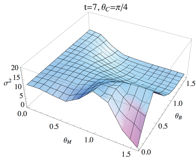
Figure 4 | Variance of the self-avoiding quantum walk with unsymmetrised input state (Eq. 10). Contrast the different dynamics with Fig. 2 where a symmetrised input state was employed. In particular, note the drastically different variance at \theta_M = \pi/2 , \theta_B = 0 compared to the symmetrised case – the maxima in the symmetrised plot corresponds to the minima of the unsymmetrised plot. Note the different viewing angle than Fig. 2.
