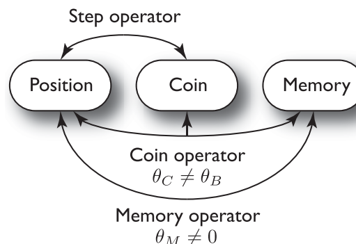
Figure 5 | Illustration of the couplings between the position, coin and memory subsystems, depending on \alpha_B , \theta_C and \theta_M . The coin operator couples all three subsystems, provided that \theta_C \neq \theta_B . The memory operator couples the position and memory subsystems, provided that \theta_M \neq 0 . The step operator couples the position and coin subsystems, irrespective of the parameters.
