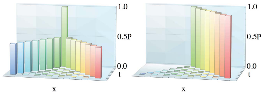
Figure 3 | Evolution of the self-avoiding quantum walk for \theta_M = \pi/2 , \theta_B = 0 , with symmetrised (left) and unsymmetrised (right) input states (Eqs. 8 and 10 respectively). This illustrates the high sensitivity of the dispersion to the initial state, as the former exhibits the maximum possible variance, whereas the latter exhibits zero variance.
