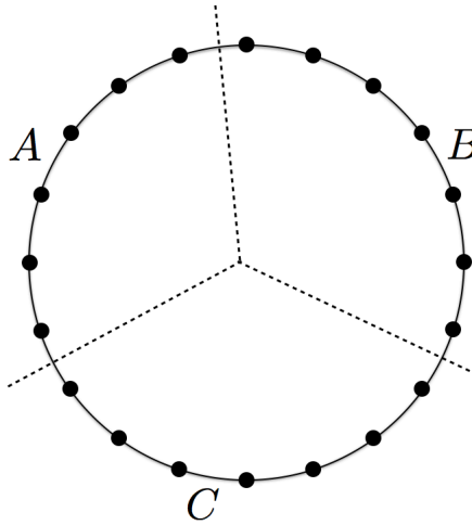
Figure 8: A, B, C cutting on a 1D ring.
