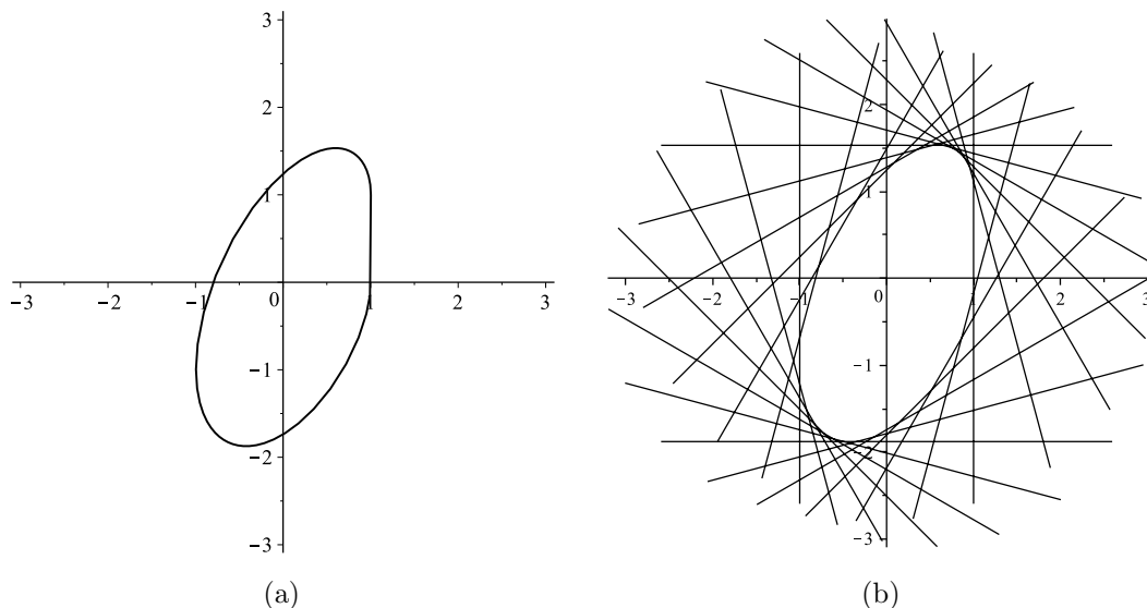
Figure 2: (a) The convex set of \mathcal{D}_{\mathcal{F}} in \mathbb{R}^2 . The horizontal axis corresponds to the value of \text{tr}(\rho F_1) and the vertical axis corresponds to \text{tr}(\rho F_2) ; (b) The supporting hyperplanes of \mathcal{D}_{\mathcal{F}} in \mathbb{R}^2 (i.e. the straight lines on the figure which are tangent to \mathcal{D}_{\mathcal{F}} ), which corresponds to the Hamiltonians H = \theta_1 F_1 + \theta_2 F_2 .
