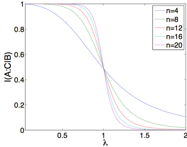
Figure 5: I(A:C|B) of the Ising model with open periodic boundary condition and the A, B, C regions as chosen in Fig. 4. A similar result is presented in [24], from a different viewpoint.
