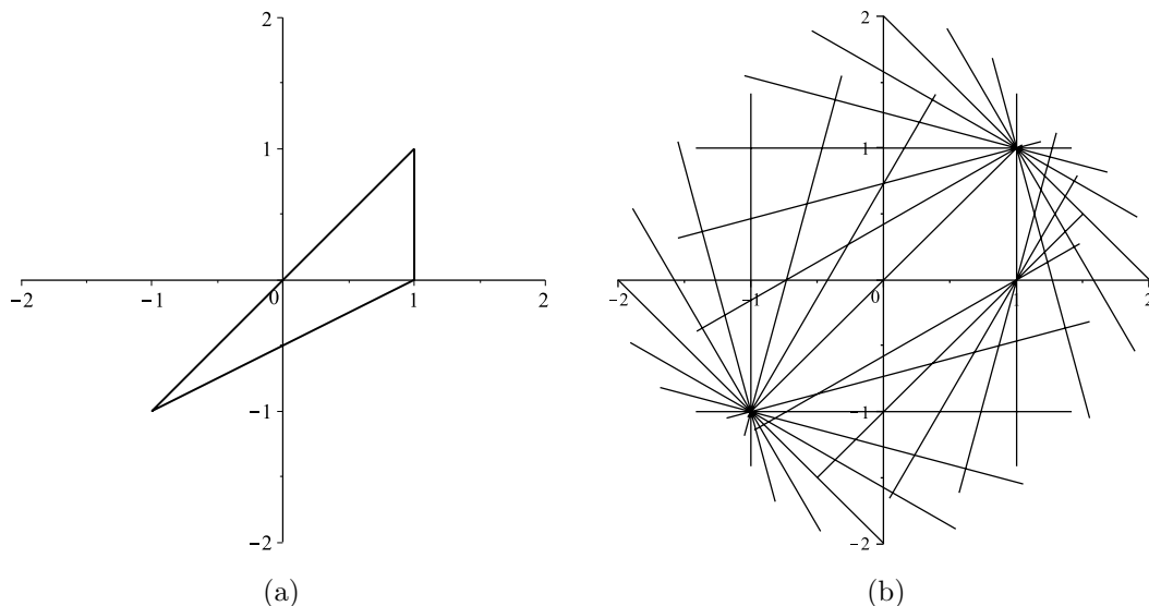
Figure 3: (a) The convex set of \mathcal{D}_{\mathcal{F}} in \mathbb{R}^2 . The horizontal axis corresponds to the value of \text{tr}(\rho F_1) and the vertical axis corresponds to \text{tr}(\rho F_2) ; (b) The supporting hyperplanes of \mathcal{D}_{\mathcal{F}} in \mathbb{R}^2 (i.e. the straight lines on the figure which are tangent to \mathcal{D}_{\mathcal{F}} ), which corresponds to the Hamiltonians H = \theta_1 F_1 + \theta_2 F_2 .
