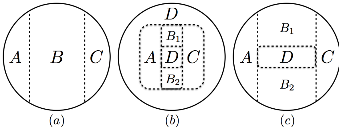
Figure 11: Cuttings on a 2D disk
