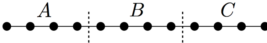
Figure 6: A, B, C cutting on a 1D chain.
