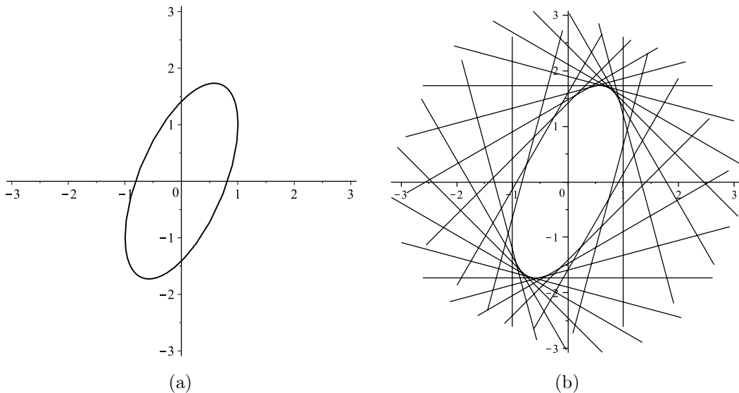
Figure 1: (a) The convex set of \mathcal{D}_{\mathcal{F}} in \mathbb{R}^2 . The horizontal axis corresponds to the value of \text{tr}(\rho F_1) and the vertical axis corresponds to \text{tr}(\rho F_2) ; (b) The supporting hyperplanes of \mathcal{D}_{\mathcal{F}} in \mathbb{R}^2 (i.e. the straight lines on the figure which are tangent to \mathcal{D}_{\mathcal{F}} ), which corresponds to the Hamiltonians H = \theta_1 F_1 + \theta_2 F_2 .
