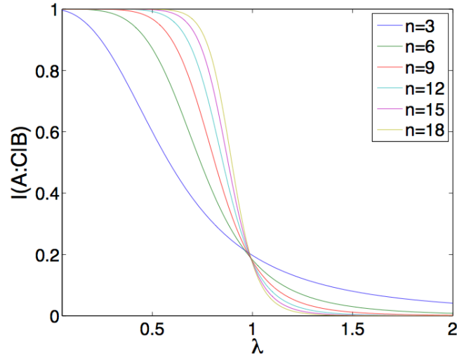
Figure 7: I(A:C|B) of the Ising model with open boundary condition and the A, B, C regions as chosen in Fig. 6.
