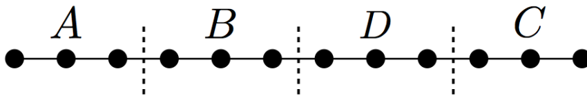
Figure 10: A, B, C, D cutting on a 1D chain
