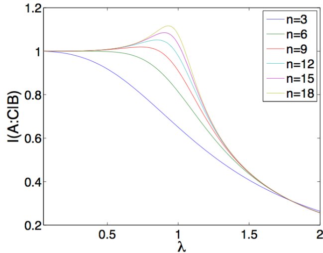
Figure 9: I(A:C|B) of the Ising model with periodical boundary condition and the A, B, C regions as chosen in Fig. 8.
