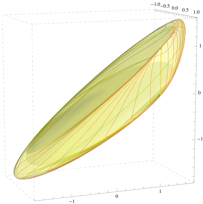
Figure 12: The convex set of \mathcal{D}_{\mathcal{F}} for \mathcal{F} = (F_1, F_2, F_3) of Example 6 in \mathbb{R}^3 . For the normalized ground state \rho(\alpha, \phi) of \cos \alpha F_1 + \sin \alpha \cos \phi F_2 + \sin \alpha \sin \phi F_3 for any given \alpha \in [0, \pi] , \phi \in [0, 2\pi] , a point is plotted for (\text{tr}(\rho(\alpha, \phi)F_1), \text{tr}(\rho(\alpha, \phi)F_2), \text{tr}(\rho(\alpha, \phi)F_3)) . Gray lines correspond to \alpha \in [0, \pi/2] , and red lines correspond to \alpha \in [\pi/2, \pi] . The yellow line corresponds to (1, 1, x) , where the discontinuity happens.
