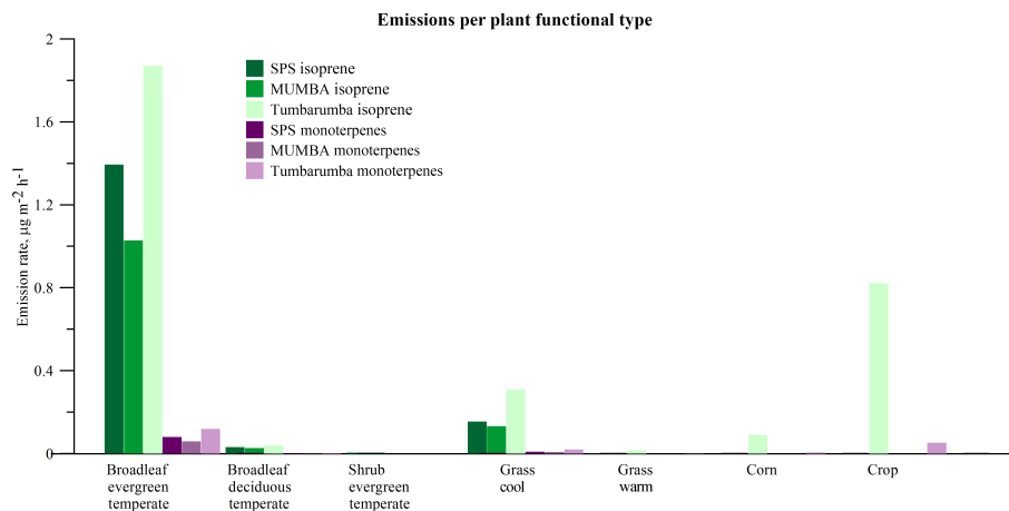
Figure 4. Emission rates of isoprene and monoterpenes per PFT within each campaign's inner domain (180 km × 180 km).
