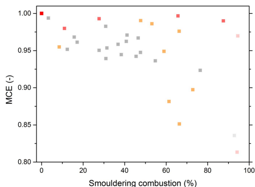
Figure 10. A scatter plot of MCE vs. the percentage area of the combusting fuel bed undergoing smouldering combustion. The same colour gradation scheme from Fig. 6 is used to denote different combustion phases. The first data point is nearly coincidental (i.e. MCE approximately 1) for all three fire spread modes, which is why only one symbol is visible.
