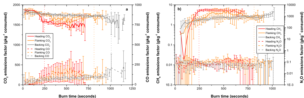
Figure 9. Time-resolved emissions factors for the trace gas emissions species measured during the experimental burns. (a) Time-resolved CO 2 and CO emissions factors. (b) Time-resolved CH 4 and N 2 O emissions factors. Coloured vertical and dotted bars represent the median end time for predominantly flaming combustion for each fire spread mode.
