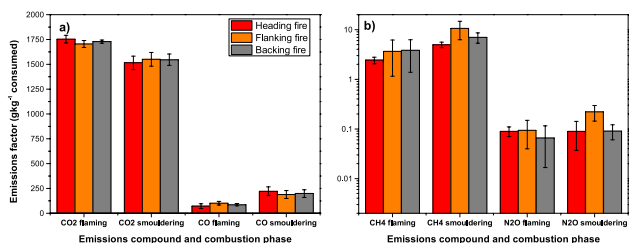
Figure 8. Carbon and nitrogen based emissions factors (per unit of dry fuel consumed) for different combustion phases within the experimental burns: (a) CO 2 and CO emissions factors for flaming and smouldering combustion; (b) CH 4 and N 2 O emissions factors for flaming and smouldering combustion.
