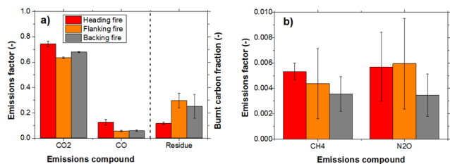
Figure 7. Carbon and nitrogen based emissions factors (per unit of carbon or nitrogen burnt) and burnt carbon residue fractions from the experimental burns: (a) CO 2 , CO and residue carbon emissions factors; (b) CH 4 and N 2 O emissions factors.
