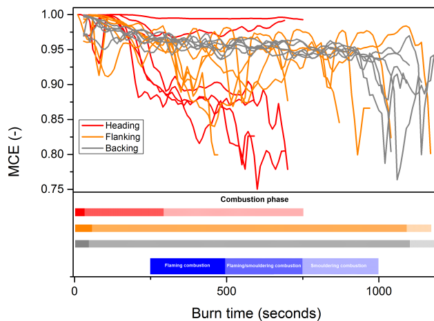
Figure 6. Time series of MCE for the experimental burns. The combustion phase for each fire spread mode is split into the duration of flaming, flaming and smouldering and smouldering combustion.
