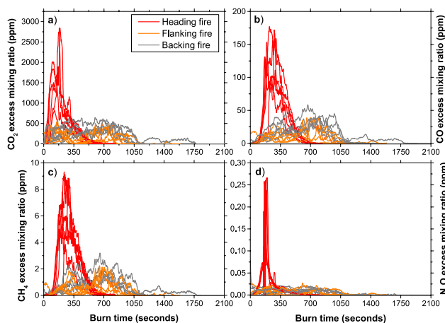
Figure 5. Time series of excess mixing ratios for different emissions species and three different fire spread modes: (a) CO 2 ; (b) CO; (c) CH 4 ; (d) N 2 O. Note that each line of a particular colour represents one experimental replicate.
