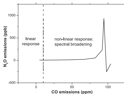
Figure 3. A graph of the interaction between \text{N}_2\text{O} and CO emissions measurements during routine calibrations which necessitated the use of a dilution system.
