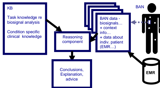
Fig. 3 CDSS with real time biosignal input from Body Area Network
