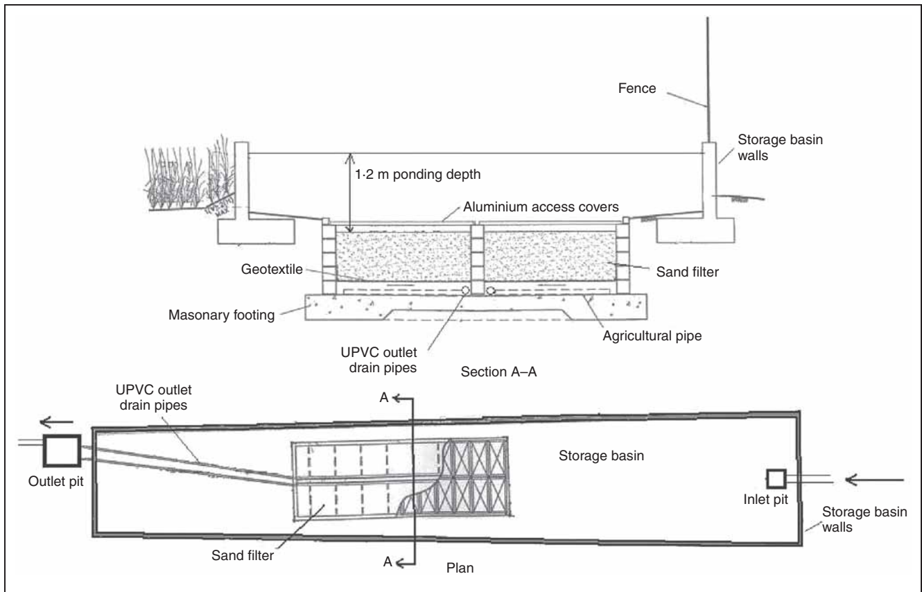
Fig. 1. Schematic view of SFD
