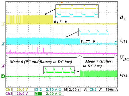
(c) PV and battery charge DC bus then PV stops to supply power (Mode 6 to Mode 7).
