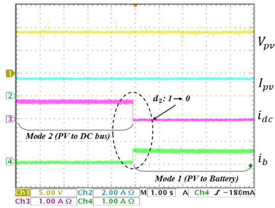
(a) Load switching for PV (Mode 2 to Mode 1).
