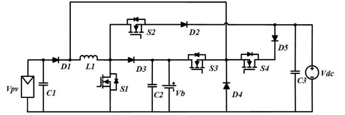
Fig. 2: Proposed converter topology.
