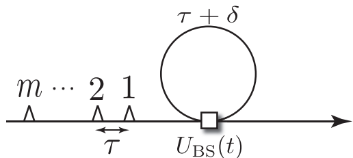
FIG. 7: The inner fiber-loop with an error \delta in its intended length. Every time a pulse traverses the inner loop it is shifted from its expected temporal position by \delta , thereby reducing the Hong-Ou-Mandel visibility at U_{BS} .
