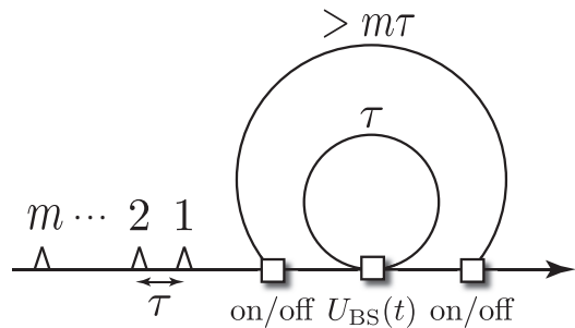
FIG. 1: The complete fiber-loop architecture fed by a pulse-train of photonic modes, each separated in time by \tau . The squares represent optical switches. A single length \tau inner fiber-loop is embedded inside a length > m\tau outer fiber-loop. The outer loop allows an arbitrary number of inner loops to be applied consecutively. When m - 1 inner loops are implemented this architecture realises an arbitrary unitary transformation on m modes given that no loss is present.
