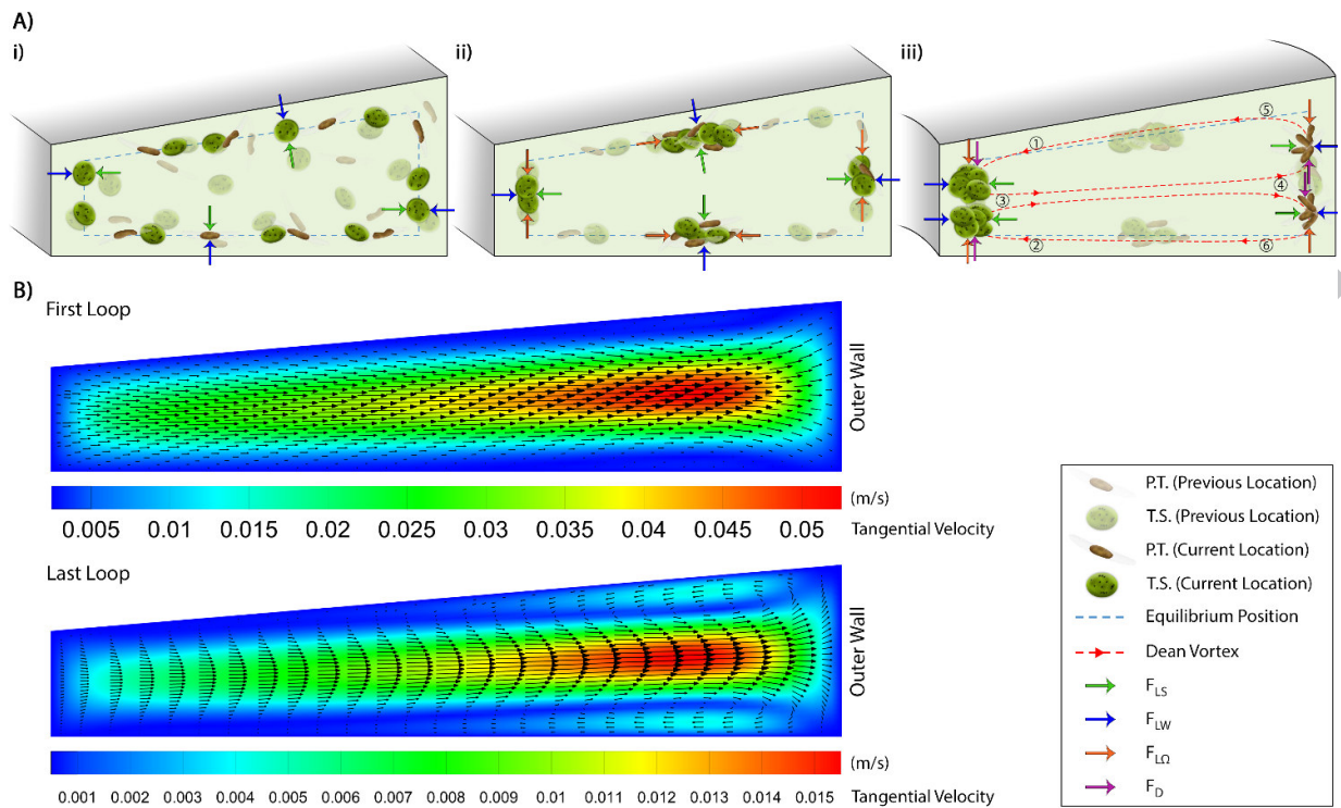
Figure 1. (A) Cross-sectional view of microalgae undergoing inertial focusing. (i) In a straight microchannel with a slanted cross-section, cells focus on equilibrium lines where F_{LS} equals F_{LW} . (ii) After travelling a longer distance, particles/cells focus on the same equilibrium lines, but also in the middle of the channel walls due to the influence of F_{L\Omega} . (iii) In a curved channel of the same cross-section, centrifugal forces act on the fluid and induce Dean flow. These secondary flow relocates the equilibrium positions of (i) and (ii) since F_{LS} , F_{LW} , F_{L\Omega} , must now also balance with a Dean drag force, F_D . (B) Tangential velocity contours obtained from numerical simulation (using ANSYS-FLUENT®) in the first and last loops of a spiral channel for the microchannel geometry used in this work. In the last loop, the secondary flow vortices in the center of the channel push particles/cells towards the outer wall. (P.T.: P. tricorutum , T.S.: T. suecica )
