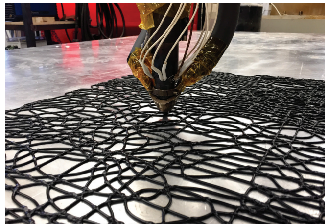
4 Robotic additive manufacturing workcell towards the beginning of the additive manufacturing process.
