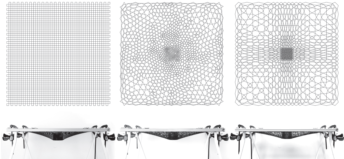
6 (Top) Plan figures and (bottom) physical deformation results of test rig cable nets: (L to R) base square-celled, optimized random uniform distribution method, and optimized subdivision method.
