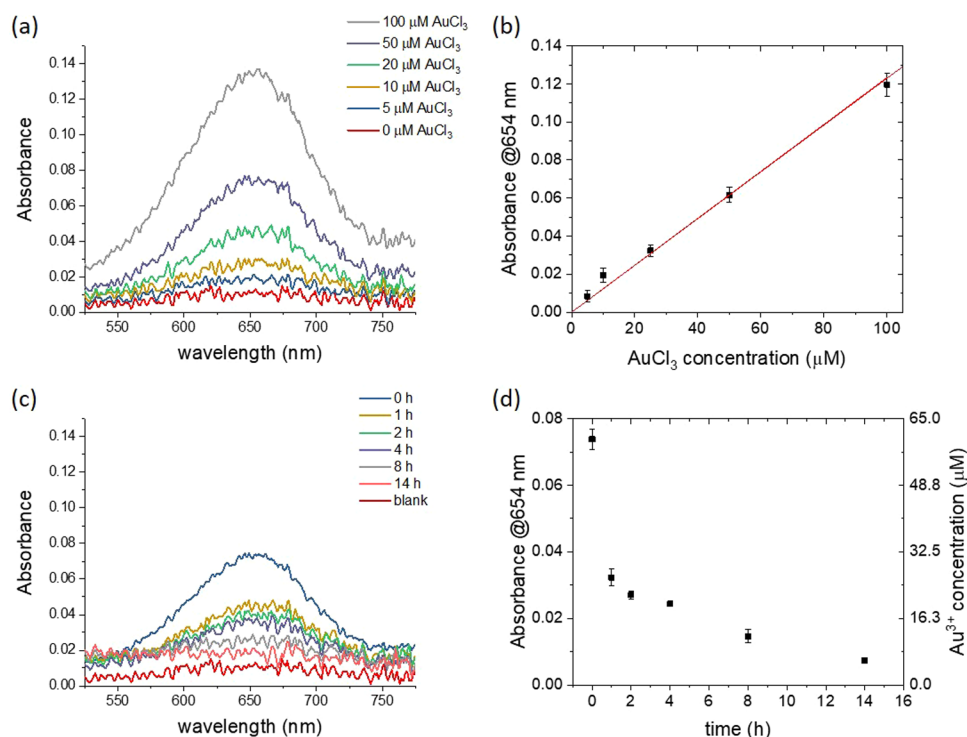
Figure 6. TMB assay to verify the gold biomineralized by D. acidovorans biofilm for 14 h. (a) Assay calibration performed on AuCl 3 samples in PBS. The reaction between gold ions and TMB molecules produces an increase in the absorbance at 654 nm, which can be used to quantify the concentration of the gold ions. (b) TMB assay calibration. (c) The D. acidovorans biofilm is stressed with 60 μM of AuCl 3 and samples of 10 μL are collected from the solution in the QCM cell. These are stored at 4 °C until the last volume is acquired at 14 h. Then, 2 μL of TMB solution is added to each sample and the absorbance spectrum in the visible range is recorded after 10 min. (d) The progressive decrease in absorbance at 654 nm documents the progressive depletion of the free ionic gold, neutralized by deltidibactin in the form of nanonuggets. Each data point corresponds to the average of the absorbance of three different samples, while the error bars denote the standard deviation.
