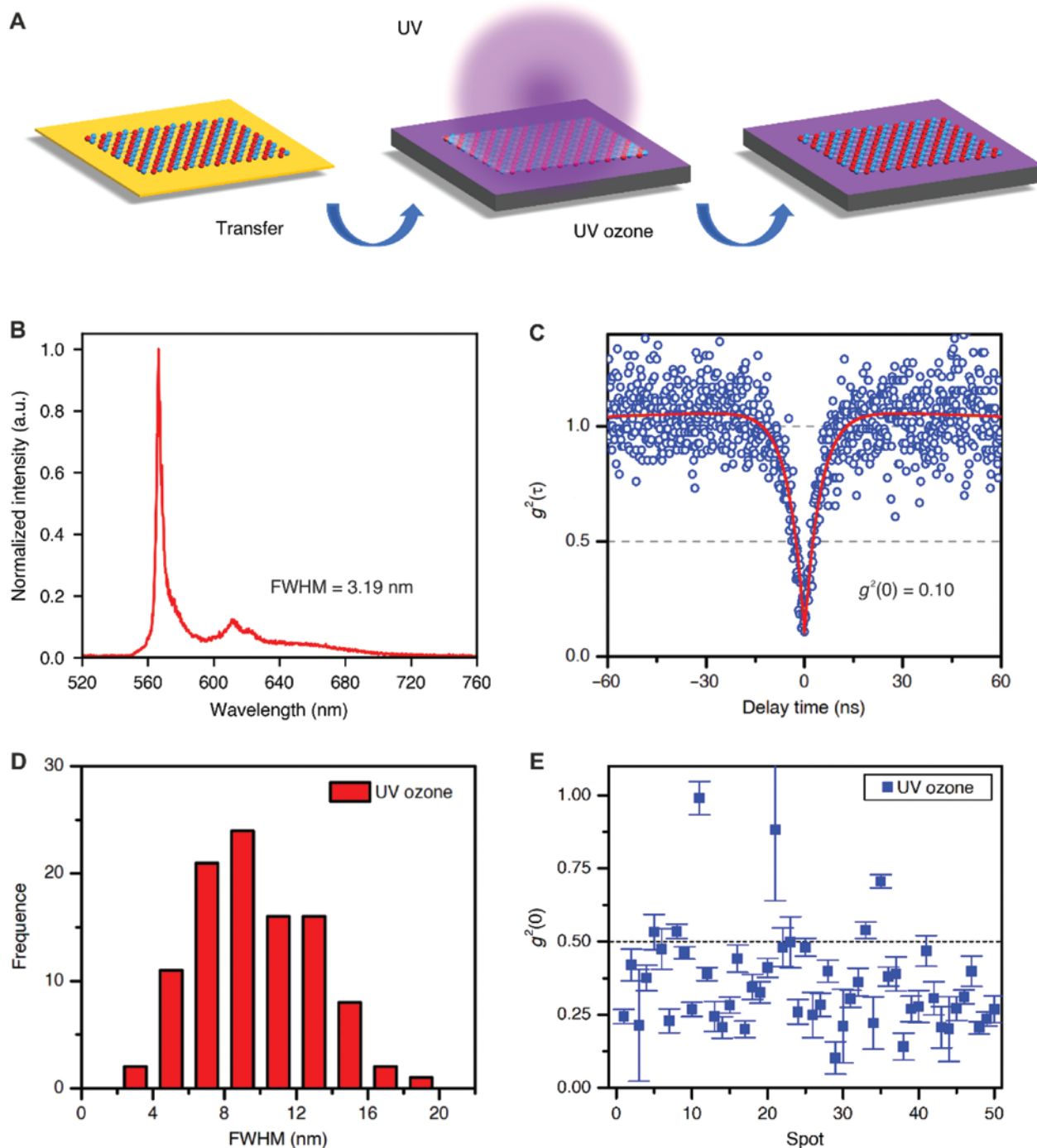
Figure 2: Room-temperature optical characterizations of hBN films that were processed by UV ozone.
