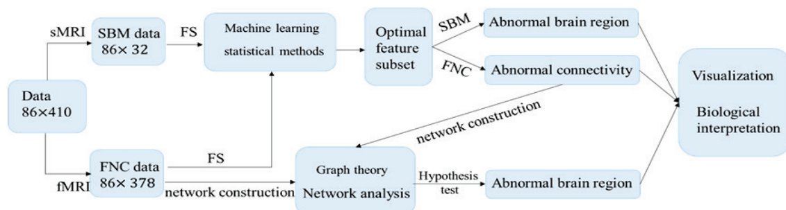
Figure 2. The flowchart of locating the abnormalities in brains for SZ. Where SBM refers to source-based morphometric, FNC refers to functional network connectivity and FS refers to feature selection.
