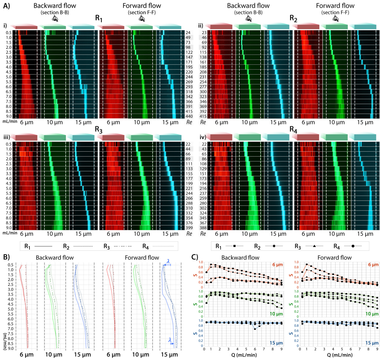
FIG. 3. Experimental results of the rectangular channels. (a) Top-view observations of fluorescent beads of 6, 10, and 15 μm diameter at Q = 0.5\text{--}9 ml/min in [(i)–(iv)] channels R_{1\text{--}4} , respectively. Note: The fluorescent color of 6, 10, and 15 μm beads is red, green, and blue, respectively. (b) Focusing positions of microbeads, regardless of how the bands are wide, at Q = 0.5\text{--}9 ml/min. (c) The sharpness factor for different particle sizes at Q = 0.5\text{--}9 ml/min.
