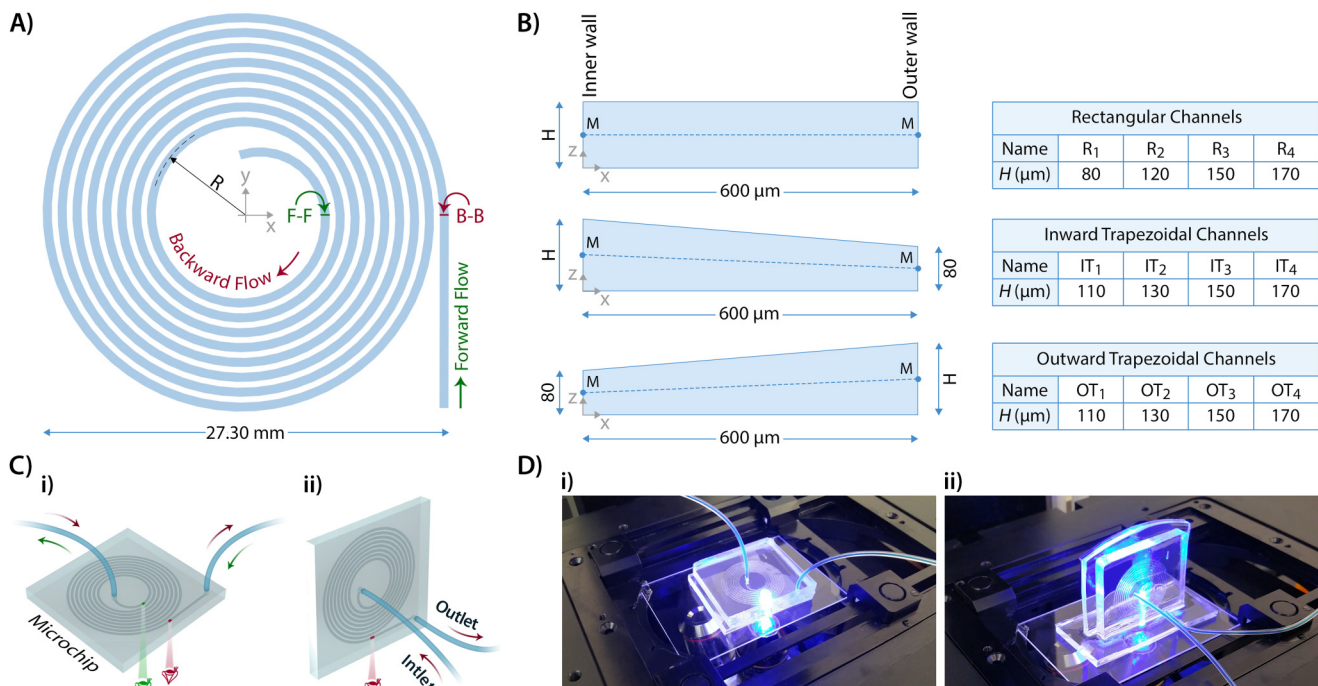
FIG. 1. Schematic of microchannels. (a) Top view of the spiral microchannels used in this study (i.e., the x - y plane). R indicates the radius of the channel curvature. Also, F-F and B-B denote sections of interest (near the outlet) in forward and backward flows, respectively. (b) Cross section of all channels in the x - z plane. The dashed “M-M” line designates the centerline of the cross section. (c) Schematic of the microchip for (i) top view observation in the forward (green) and backward (red) flows, and (ii) side-view observation in the backward flow. (d) Images of the experimental setup for an inverted microscope (i) top view and (ii) side view.
