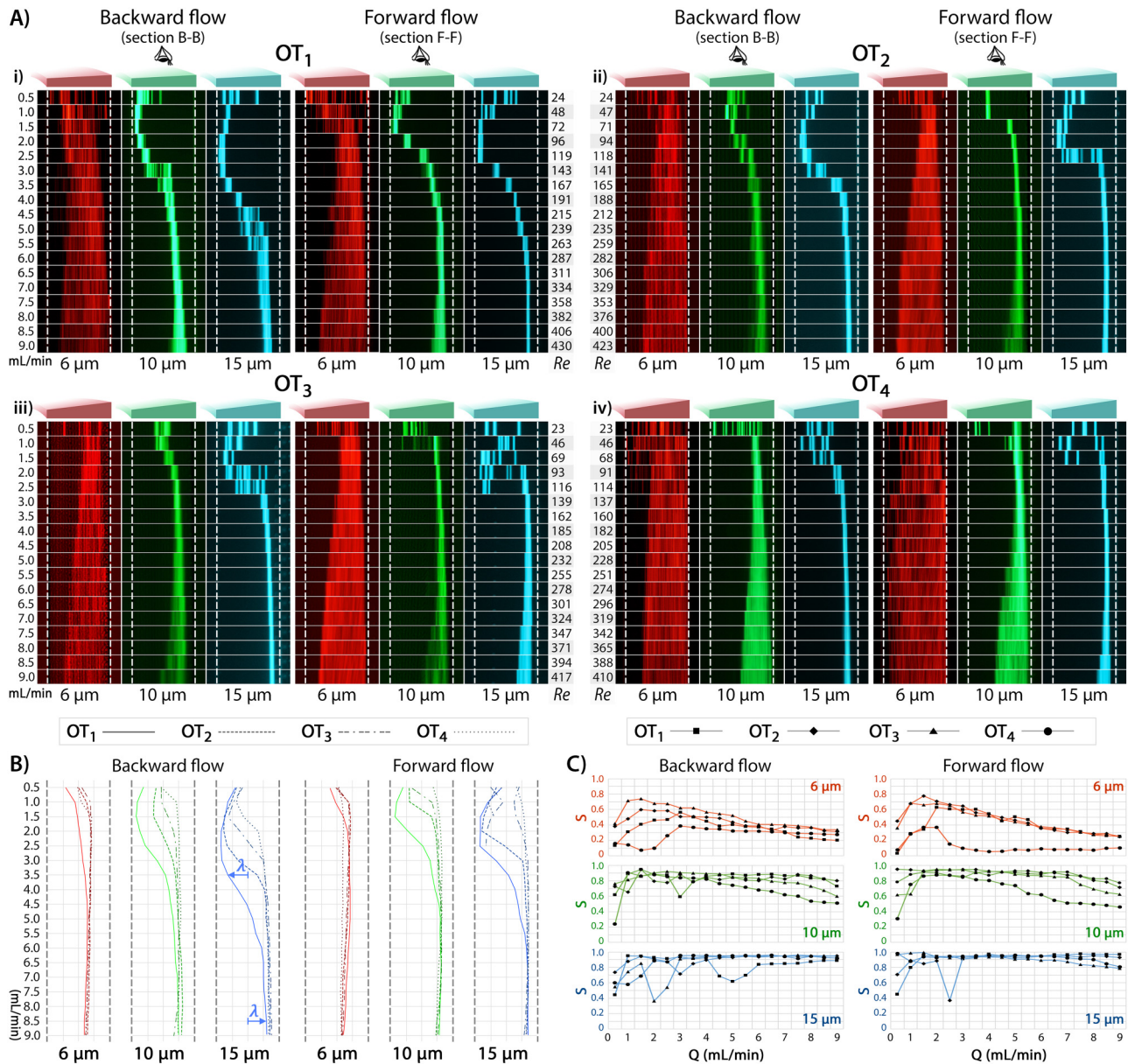
FIG. 7. Experimental results of the OT channels. (a) Top-view observations of fluorescent beads of 6, 10, and 15 μm diameter at Q = 0.5\text{--}9 ml/min in [(i)–(iv)] channels OT 1–4 , respectively. (b) Focusing positions of microbeads, \lambda , at Q = 0.5\text{--}9 ml/min. (c) The sharpness factor for different particle sizes at Q = 0.5\text{--}9 ml/min.
