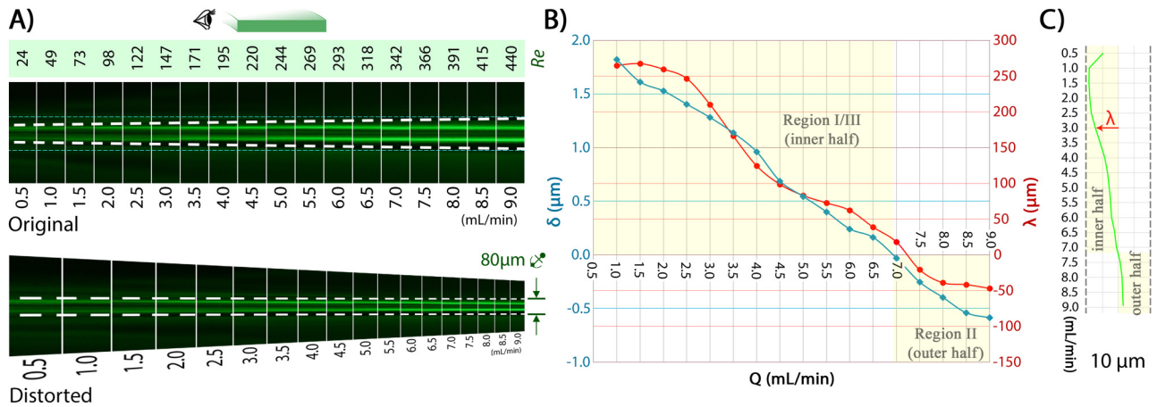
FIG. 4. Approach of particles to the M-M centerline. (a) Original and linearly distorted side-view images of 10\ \mu\text{m} beads at Q = 0.5\text{--}9\ \text{ml/min} in the backward flow of the channel R_1 . Very fine dashed blue lines drawn near the top and bottom walls in the original image are horizontal lines. In the distorted image, the channel height is fixed at all the flow rates. (b) Variations of the distance ( \delta ) experimentally measured between the mean of the focusing position of 10\ \mu\text{m} particles in the channel R_1 and their nearest numerically obtained IPs, as discussed in Sec. 5 of the supplementary material . \lambda indicates the distance between the focusing band and the middle of the channel. Note that channel deformation effects inertial focusing and may add error to the measurement of \delta , as discussed in Sec. 5 of the supplementary material . (c) The top-view focusing trends of the particles at the same flow rates. Notice that the focusing band switches from the inner half to the outer half at Q = 7\ \text{ml/min} where \delta \approx 0 .
