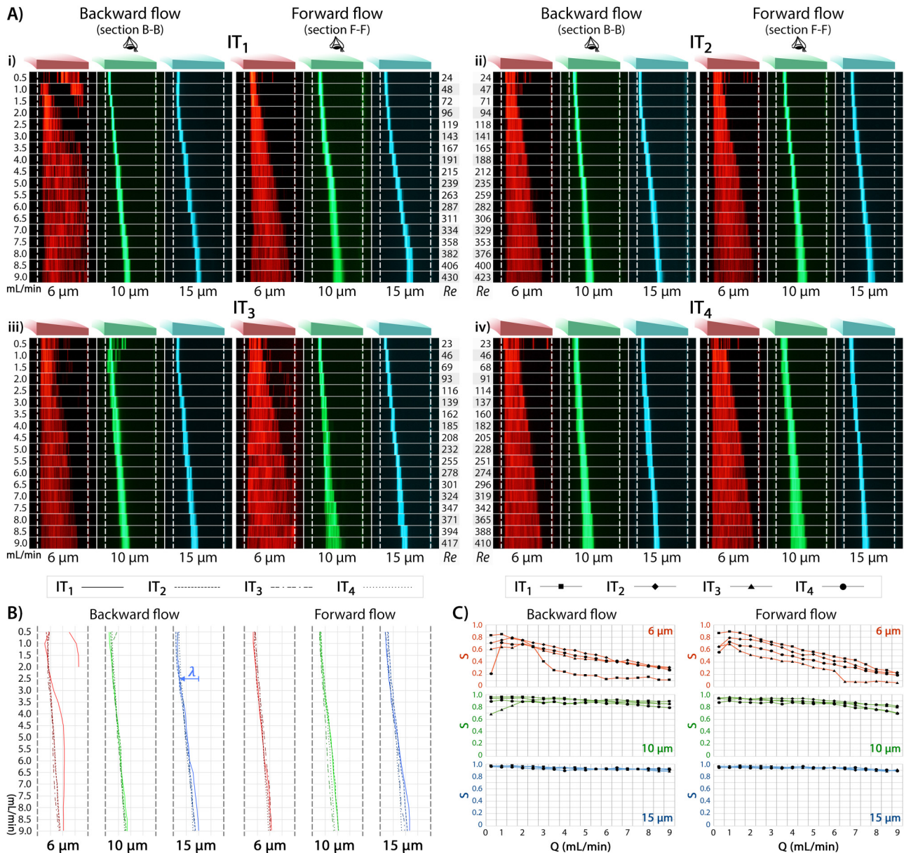
FIG. 9. Experimental results of the IT channels. (a) Top-view observations of fluorescent beads of 6, 10, and 15 μm diameter at Q = 0.5\text{--}9 ml/min in [(i)–(iv)] channels IT 1–4 , respectively. (b) Focusing positions of microbeads, \lambda , at Q = 0.5\text{--}9 ml/min. (c) The sharpness factor for different particle sizes at Q = 0.5\text{--}9 ml/min.
