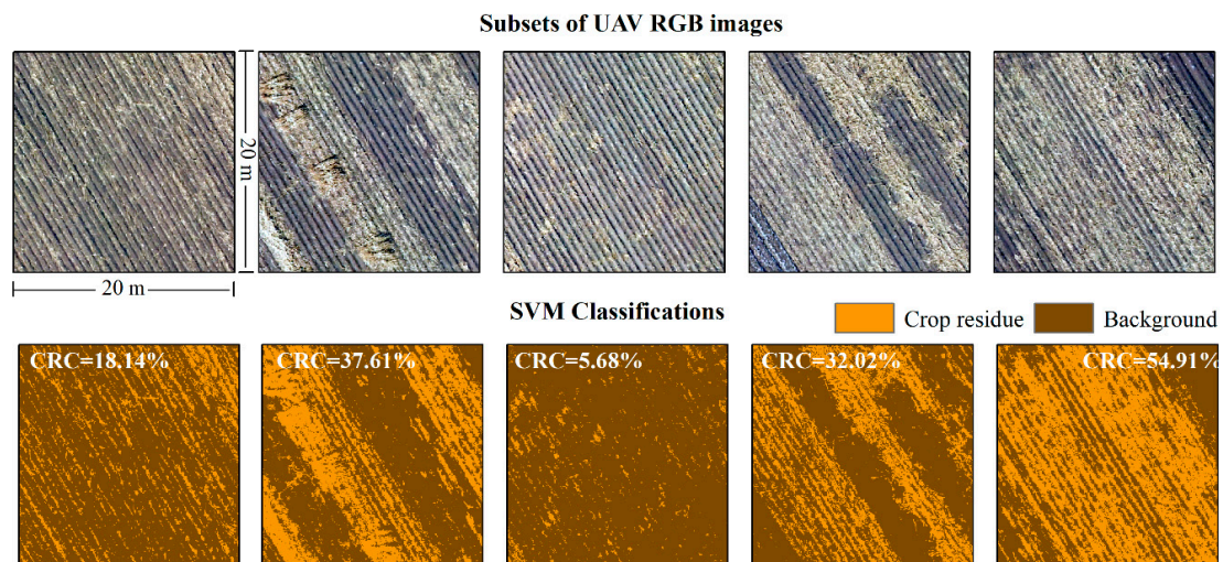
Figure 3. Examples of support vector machine (SVM) classification results. The upper figures are subsets of UAV mosaic and the lower figures are corresponding classifications.
