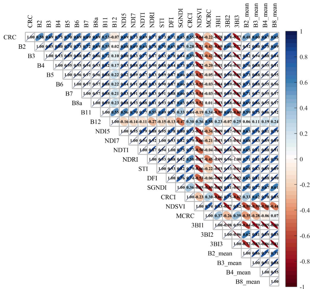
Figure 4. Correlation matrix for CRC and predictor variables including MSI bands, indices and textural features. The Sentinel-2 MSI bands are represented as B2, B3, . . . , B12. The mean textural feature are represented as B2_mean, B3_mean, . . . , B8_mean. The length on the minor axis of the ellipse indicates the strength of the Pearson’s correlation coefficient between each pair variables, while the colors of the ellipse indicate whether the correlation is positive or negative.
