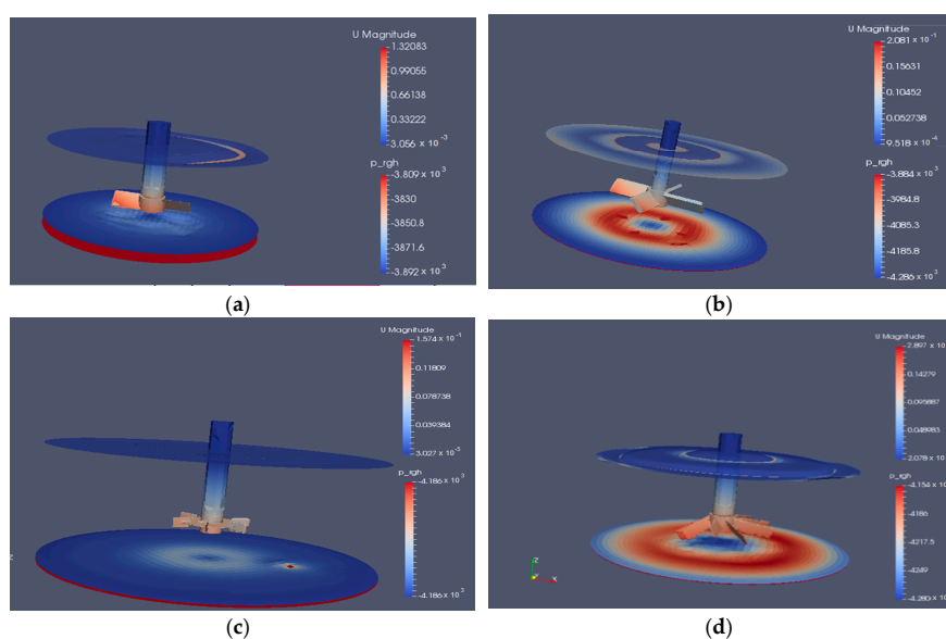
Figure 4. Isosurface comparing water interfaces for four different impellers including (a) a three-blade turbine, (b) a four-blade turbine, (c) a Rushton turbine, and (d) an eight-blade turbine.
