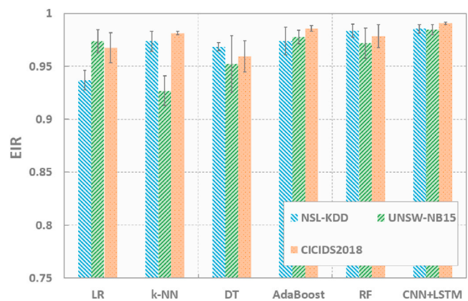
Fig. 5. Evasion increase rates of baseline algorithms.
