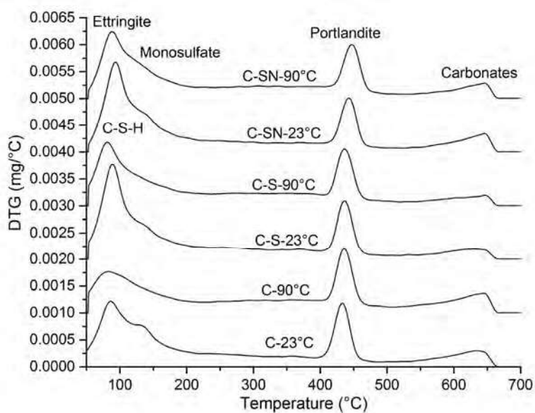
Figure 5: DTG curves of 30 days old cement pastes
