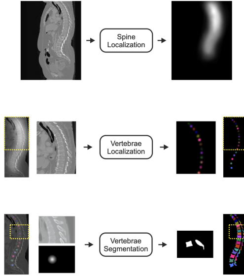
Figure 3: The three processing stages in Payer C. for localisation, identification, and segmentation of vertebrae.
