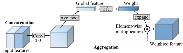
Figure C.24: Huang et al. Feature Aggregation block
