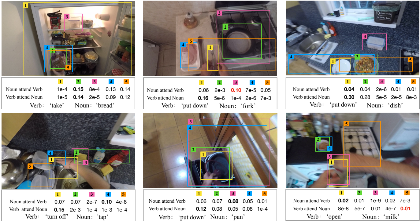
Fig. 4. Qualitative results of our SAOA I3D (Flow) model. The colored boxes show the top-5 detected regions and the numbers are the corresponding attention weights generated by our action-attended relation module. Red indicates the failure case.
