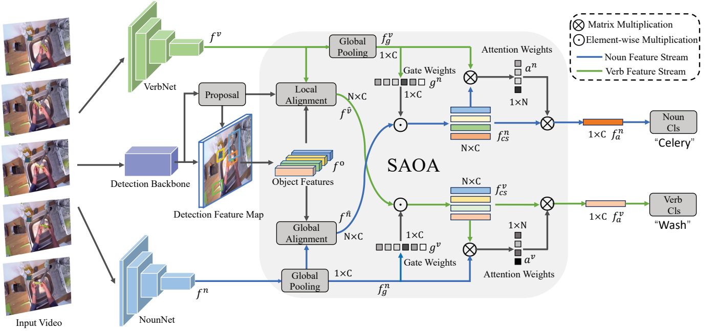
Fig. 2. The proposed SAOA framework. Our framework consists of three feature extractors and one interaction module. The detection model generates a set of local object features and location proposals. This location-aware information is injected to the two branches by an object-centric alignment method. For the Verb branch, the feature map is locally aligned with the objects by combining the local motion features with corresponding object detection features. For the Noun branch, the object features are aligned with the global noun representation. Subsequently, the fused features from each branch interact with the global feature from the other branch by a symbiotic attention mechanism. The two object-centric feature matrices are first normalized by a cross-stream gating operation. After that, the matrices are attended by the other branch to select the most action-relevant information. The outputs of SAOA are used to classify the verb and noun, respectively.
