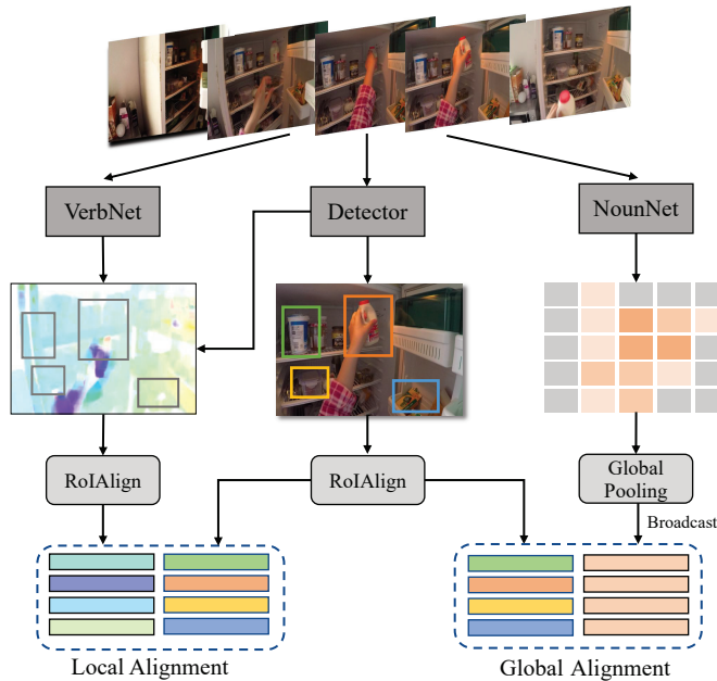
Fig. 1. The illustration of the object-centric feature alignment. For verb classification, the spatial location provided by the detector can possibly reduce the object-irrelevant motions. Local motion features aligned with object features serve as possible action candidates. For noun classification, global alignment injects the local object features into the context-aware global feature. These location-aware feature candidates from the two branches are beneficial to the subsequent meticulous reasoning.
