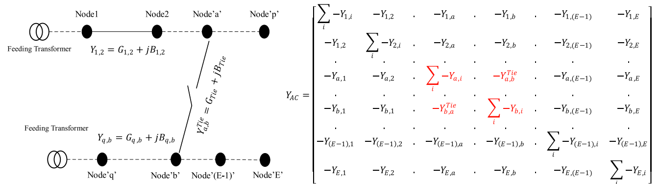
FIGURE 3 Generic view of a radial distribution network with Tie switches considered for formation of the Y_{AC} matrix
