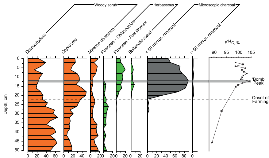
Figure 4. Preservation of the ^{14}\text{C} bomb peak and evidence of human activity in the Homestead Scarp peat sequence, subantarctic Campbell Island. Summary pollen diagram from Homestead Scarp 38,50 ; pollen values calculated as percentage total native terrestrial pollen. Dotted line marks commencement of sheep farming (CE 1931) as indicated by onset of burning and rise of unpalatable species; grey bar denotes the ^{14}\text{C} 'bomb peak'.
