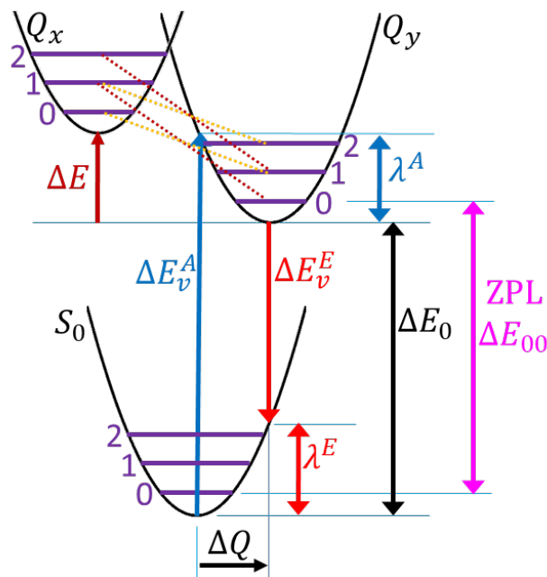
Figure 2. Critical aspects pertaining to the Q -band spectra of chlorophylls sketched on potential-energy surfaces (energy versus a generalized geometrical variable). Vibrational levels correspond to 0, 1, and 2 vibrations present in just one of the many normal modes of vibration of each state are shown. Emphasized are labels descriptive of Q_y spectroscopy: the geometry difference between the adiabatic state minima \Delta Q , the vertical absorption and emission energies, \Delta E_v^A and \Delta E_v^E , respectively, the associated reorganization energies \lambda^A and \lambda^E , the adiabatic transition energy \Delta E_0 , and the energy of the ZPL origin \Delta E_{00} . Also marked is the adiabatic energy gap of Q_x from Q_y \Delta E , and the non-adiabatic couplings indicated by dashed lines that link specific vibrational levels of Q_x and Q_y .
