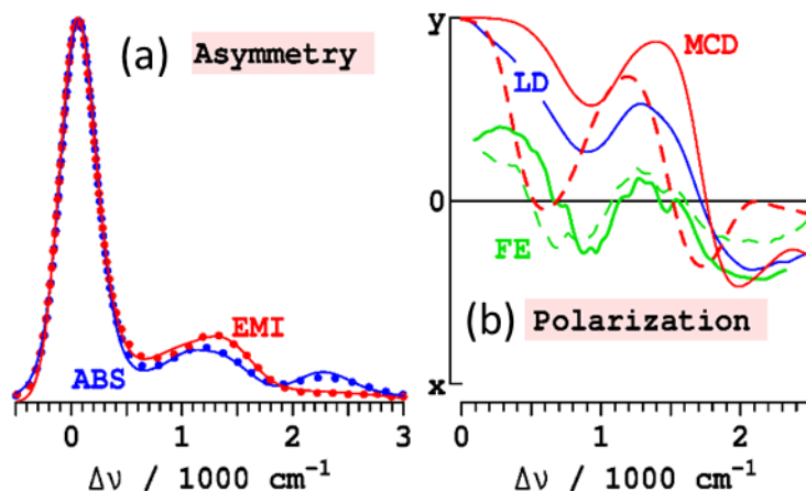
Figure 6. Observed and interpreted low-resolution spectra for Chl-a in ether at 295 K. (a) Asymmetry between the 5CO absorption A(\Delta\nu)/\nu and reflected emission E(-\Delta\nu)/\nu^3 spectra from experiment [125] (dots) and from a model including non-adiabatic coupling between Q_x and Q_y [63] (solid lines). (b) Spectral polarizations deduced for 5CO (solid lines) and 6CO (dashed lines) from experimental data [63]: blue- LD [48], red- from analytical data inversion of MCD and absorption spectra [50], green- from polarized fluorescence excitation (FE) [42] interpreted using the Q_x - Q_y non-adiabatic coupling model.
