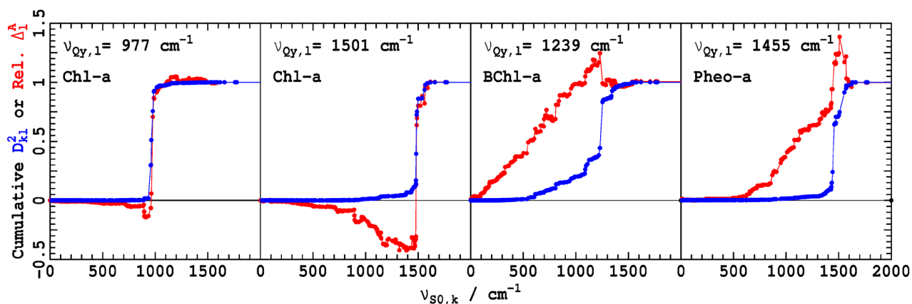
Figure 9. From Eqn. (9), the cumulative weighting from the Duschinsky matrix D_{kl}^2 , in blue and the relative contribution to the displacement \Delta Q_l^A that describes the intensity of line l in absorption in terms of contributions from each ground-state mode k , in red [67,122,124].
