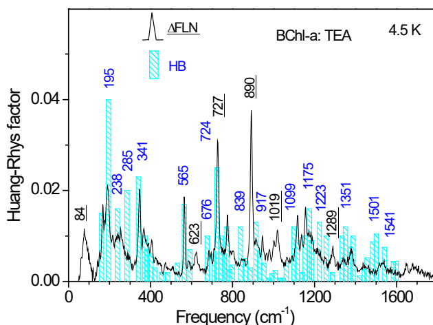
Figure 5. Comparison of the 6CO BChl-a mode structures related to the Q_y transition, as observed at 4.5 K by \Delta FLN (black curve) [67] and SHB (turquoise histogram) [123] methods. The numbers indicate the main vibrational frequencies in wavenumbers. Reprinted with permission from ref 67. Copyright 2011 AIP Publishing.
