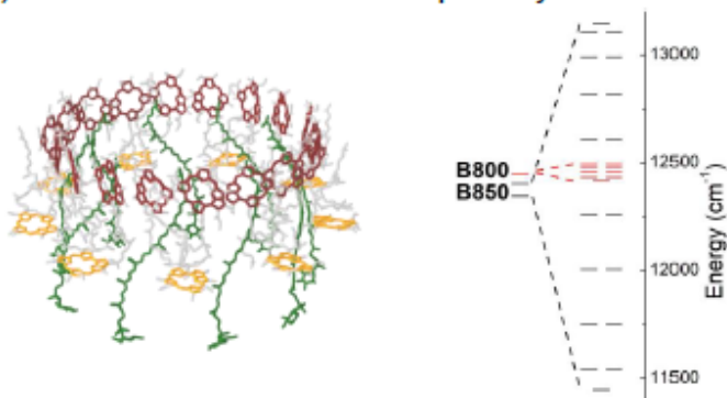
Figure 1. Bacteriochlorophyll-a (BChl-a) in different environments: gas phase (a) [66]; solid solution of 1-propanol (b) [67]; and LH2 light-harvesting pigment-protein complex from Rhodoblastus acidophilus (c) [68]. Shown for simplicity in the latter structure are only pigment molecules: 27 BChl-a (drawn by dark red and yellow colors) and 9 carotenoids (green). See text for further explanations.
