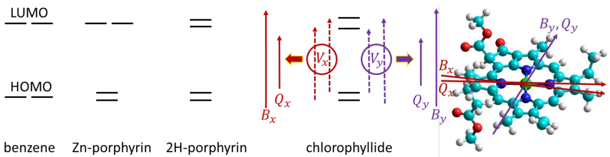
Figure 2. Basic Gouterman model for the spectroscopy of porphyrins and chlorophylls and its relationship to benzene and the acenes. Increasing degrees of asymmetry split the doubly degenerate HOMO and LUMO orbitals of benzene, with the visible-region spectroscopic transitions Q_y , Q_x , B_y , and B_x (solid arrows) arising following strong configuration interaction V_x and V_y between pairs of the embodied single-electron transitions (dashed arrows). The directions of the associated (approximately in plane) transition dipole moments calculated by CAM-B3LYP are indicated on the molecular model for methyl-Chl-a: C- cyan, H- white, N- blue, O- red, Mg- green.
