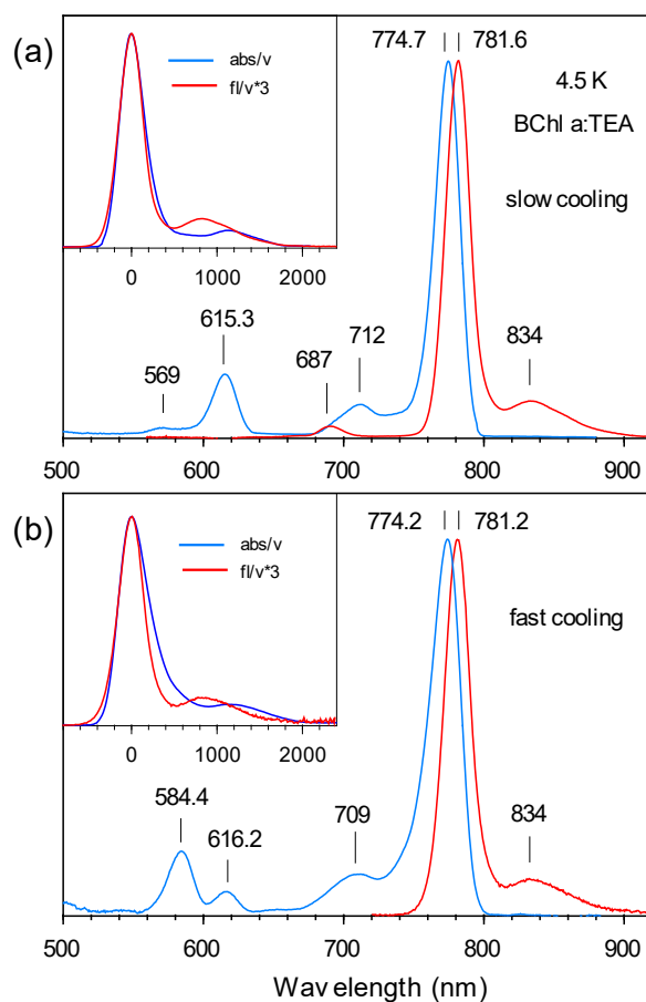
Figure 4. Absorption (blue line) and fluorescence (red line) spectra at 4.5 K of BChl-a in (a) hexa-coordinated TEA following slow cooling and (b) mostly penta-coordinated TEA following rapid cooling. The fluorescence spectra were excited at around 405 nm. The vertical lines label band positions in nanometers. The insets show the overlap of the absorption and emission spectra in transition dipole moment representation as a function of the frequency differences \nu - \nu_{00} for absorption and \nu_{00} - \nu for emission in wavenumbers. Reprinted with permission from ref 67. Copyright 2011 AIP Publishing.
