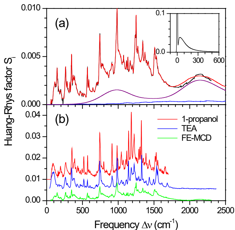
Figure 7. (a) The normalized high-resolution fluorescence excitation spectrum of Chl-a in wet ether at 4.2 K [42] (black) and its interpretation (red). The fitting curve is evaluated as a sum of a low-resolution x -polarized component (purple, obtained self-consistently along with the MCD spectral fit) and a 236-mode Huang-Rhys component with assumed ZPL and PSB spectral shape (inset). The blue curve shows the contribution of multiple excitations to the Huang-Rhys spectrum [63]. (b) Comparison of the Chl-a mode structures in 1-propanol (red) and TEA (blue) related to the Q_y transition, as observed at 4.5 K by \Delta FLN, with the y -polarized fluorescence excitation profile obtained by subtraction of the purple x -polarized component from the black experimental fluorescence excitation spectrum, as shown in panel (a). The three curves are for better visibility vertically shifted relative to each other by 0.005 units. For both (a) and (b), the y -scale is such that the value of the Huang-Rhys factor for a vibrational fundamental that is not overlapped by other peaks is given by the peak height.
