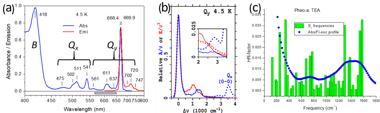
Figure 3. Aspects of the absorption and emission spectra of Pheo-a in TEA glass at 4.5 K. (a) Unscaled low-resolution spectra, discernible into contributions from the Soret bands B as well as the Q_x and Q_y bands. (b) The Q_y spectra shown as deviations \Delta\nu = \nu - \nu_{00} in absorption ( A ) and \nu_{00} - \nu in emission ( E ), normalized to produce the band-shape functions A/\nu and E/\nu^3 (dots), and their fit to a Huang-Rhys model (solid lines). (c) absorption-type spectra prepared as for (b), except the band-shape function is quantified as an effective Huang-Rhys factor (this is accurate only if bands are non-overlapping) depicting low-resolution and high-resolution fluorescence excitation spectra. Adapted with permission from ref 122. Copyright 2019 AIP Publishing.
