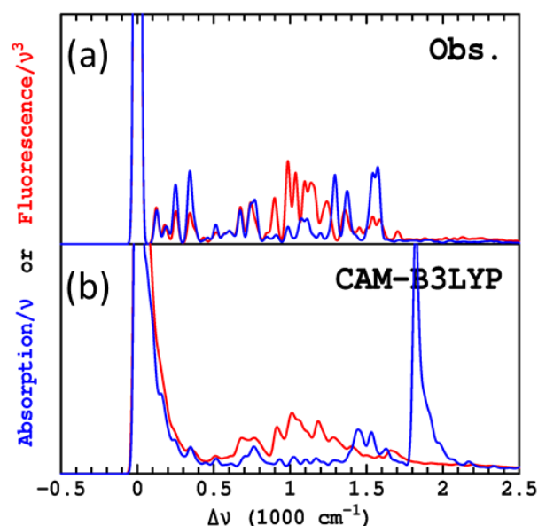
Figure 10. Observed (in TEA at 4.5 K) and calculated (CAM-B3LYP, gas phase) high-resolution spectra, depicting absorption (blue) and reflected emission (red) for Pheo-a [122]. Both observed and calculated spectra are slightly broadened to avoid accidental resonance effects.
