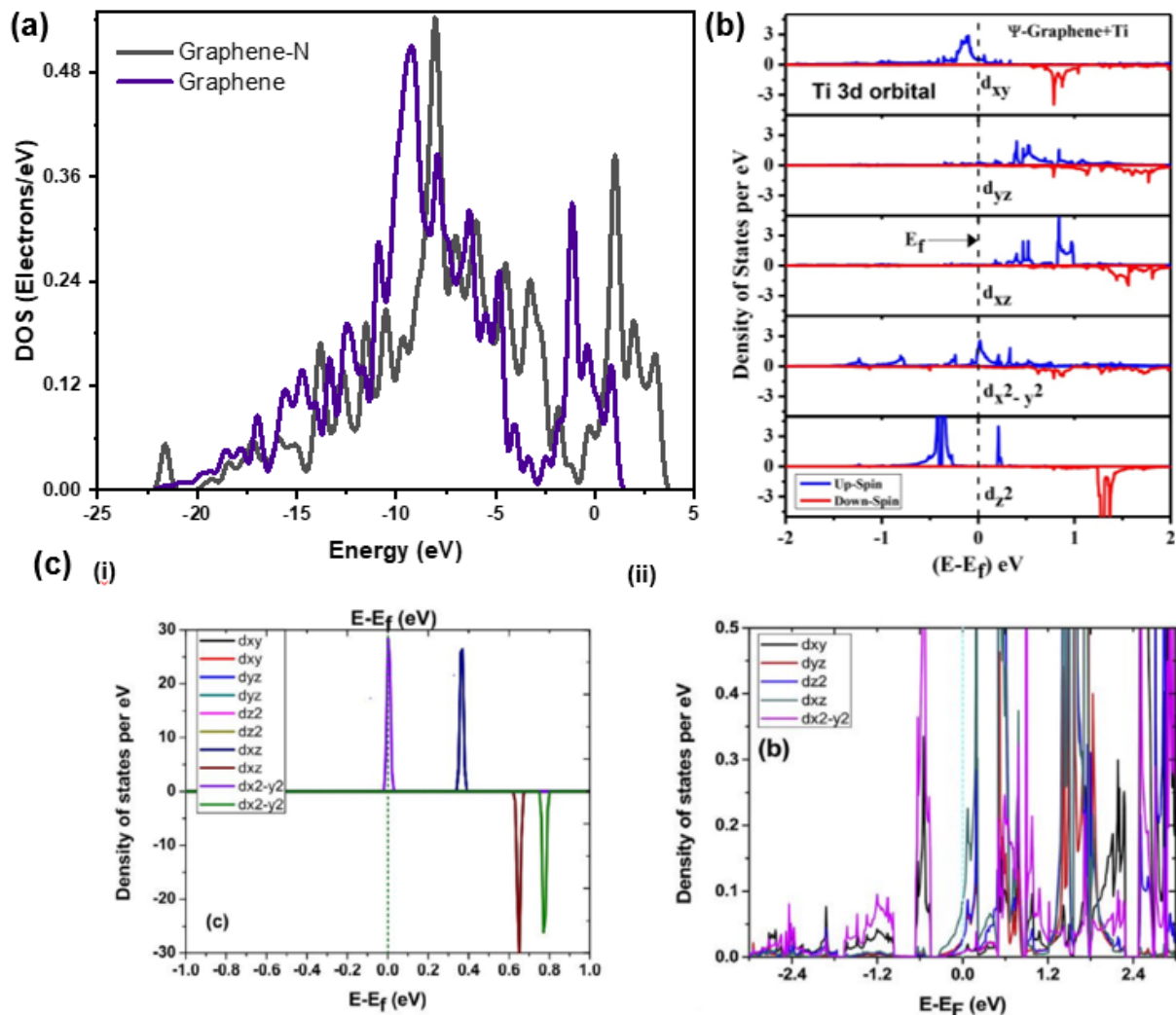
Fig. 8: (a) The PDOS plots of density of states of C-2p orbital for Graphene and N-doped Graphene. (b) Partial Density of States of sub-orbitals d_{xy} , d_{yz} , d_{z^2} , d_{xz} , and d_{x^2-y^2} of the 3d atomic orbital of Ti in \Psi -graphene +Ti 128 . (c) PDOS of (i)d orbitals of isolated Y atom; and (ii) Y d orbitals for graphyne-Y system 127 .
