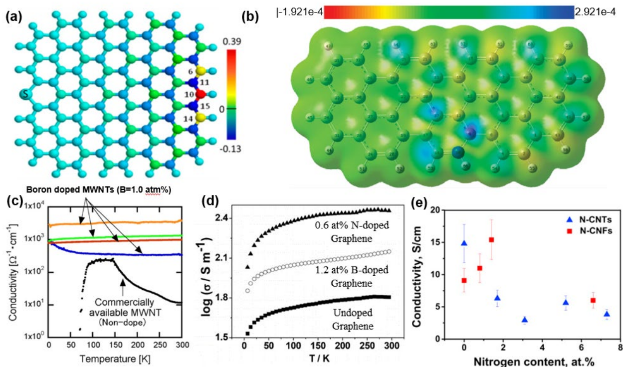
Fig. 6. (a) Spin density distributions on S-doped graphene at the zigzag edge 101 . (b) spin density distribution on the N-graphene with pyridine structure ( C_{45}NH_{20} ) 102 , The electron density isovalue plane displays the distribution of spin density; the most negative value is represented by red, and the most positive by blue. (c) Boron-doped MWNTs show higher conductivity than commercially available MWNTs, even at very low temperatures 104 . (d) Temperature dependences of electrical conductivity of N- and B-doped graphene 10 . (e) Dependence of electrical conductivity on the nitrogen content in N-CNTs and N-CNFs 105 .
