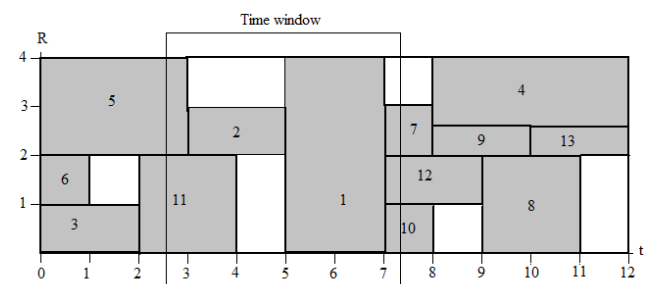
Fig. 1. An RCPSP example.
