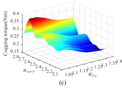
Fig. 4. Cogging torque waveforms, (a) waveform related with W_{PM\theta} and W_{FPMz} , (b) standardization waveform, and (c) standardization waveform related with W_{PM} and W_{mpw\theta} .
