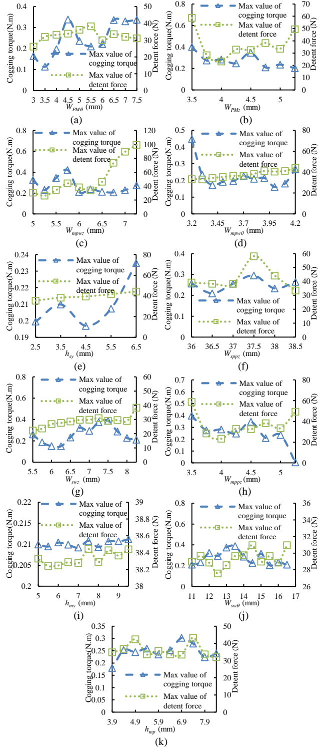
Fig. 2. Amplitude waveforms of cogging torque and detent force of the selected parameters. (a) W_{PM\theta} , (b) W_{FPMz} , (c) W_{mpwz} , (d) W_{mpw\theta} , (e) h_{sy} , (f) W_{sppz} , (g) W_{swz} , (h) W_{mppz} , (i) h_{my} , (j) W_{sw\theta} , (k) h_{mp} .
