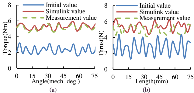
Fig. 8. The comparison waveforms of Torque/thrust, (a) torque waveforms, (b) thrust waveforms.
