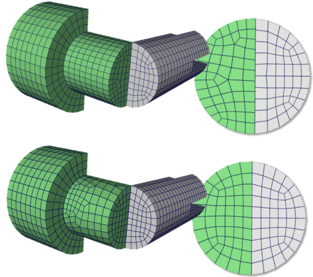
Fig. 23. Two meshes generated using sweeping are not conform along a contact surface (top); Performing sheet operations on the green mesh allows to get a conforming interface (bottom).
