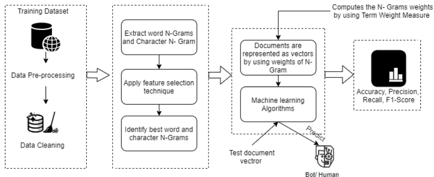
Fig. 1 The N-Gram based approach for Bot Detection
