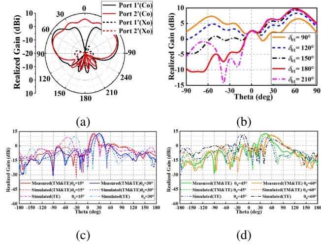
FIGURE 20. Radiation patterns of a dual-mode element and the beam scanning patterns of a 1 \times 4 -element 0.95\lambda -spaced linear array in [129]. (a) radiation pattern of the dual mode (TE and TM modes) antenna. (b) the element patterns when its two modes are fed with equal amplitudes but different phase differences. (c) and (d) show the array pattern with scanning angles of 15^\circ , 30^\circ , 45^\circ , and 60^\circ with grating lobe cancellation. Patterns with the elements all working at TE mode are also shown for comparison.
