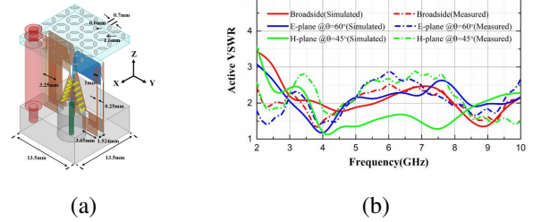
FIGURE 15. Structure of the tightly coupled dipole array (TCDA) unit cell with a metasurface WAIM layer reported in [96] (a), and (b) the VSWRs of a center element in a 16 \times 16 -element planar array for different scanning angles.
