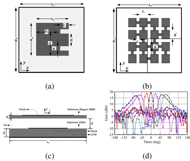
FIGURE 10. Structure of the reported antenna in [65] and the array beam scanning patterns. (a) Lower layer. (b) Upper layer. (c) Side view. (d) Beam scanning patterns of an 8 \times 8 -element array in xoz -plane.
