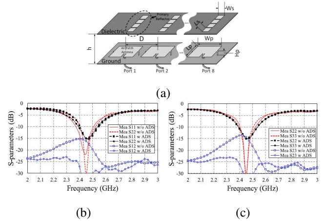
FIGURE 18. Eight-element patch antenna array with a designed ADS for mutual coupling reduction (a) and the representative measured S-parameters of the array with and without the ADS of (b) antennas 1 and 2 and (c) antennas 2 and 3 [114].
