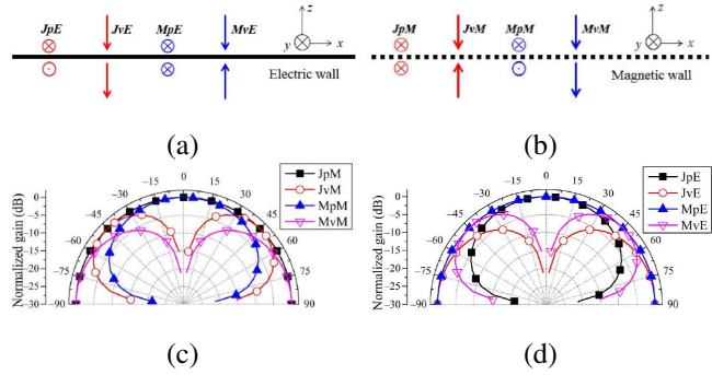
FIGURE 4. Eight basic types of image based antennas with (a) a PEC ground and (b) a PMC ground, and the corresponding theoretical radiation patterns (c) and (d) [49].
