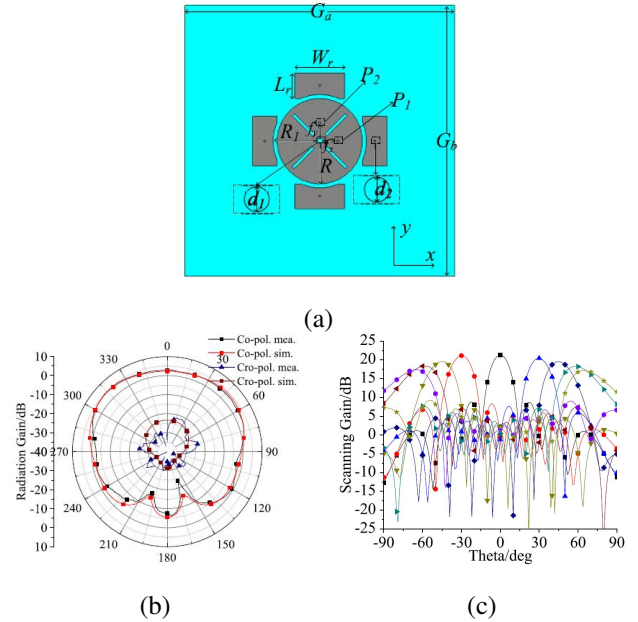
FIGURE 9. Top view of the antenna (a) reported in [62], and (b) its radiation patterns as well as (c) the simulated beam scanning patterns of the constructed 8 \times 8 -element planar array at xoz-plane.
