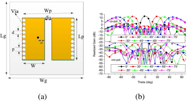
FIGURE 6. Structure of the developed magnetic dipole antenna (a), and (b) the measured WABS radiation patterns for the constructed 9-element E-plane array in [55].
