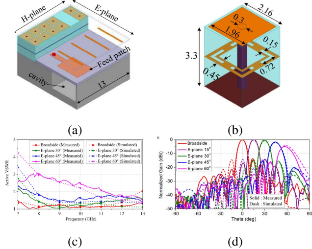
FIGURE 16. Geometries of the reported unit with EBGs and the corresponding element and array performances [110]. (a) 3-D view of the unit, (b) 3-D view of the EBG unit, (c) measured and simulated active VSWRs of a central element, and (d) the E-plane scanning patterns of a 13 \times 5 -element triangular-distributed array at 10 GHz.
