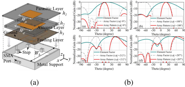
FIGURE 21. The null scanning antenna as well as the element and array patterns presented in [130]. (a) exploded view of the null scanning antenna, and (b) the element pattern and array patterns of a 4 \times 4 -element 0.8\lambda -spaced planar array with different scanning angles. (b) also shows the array factor with isotropic element pattern as a comparison.
