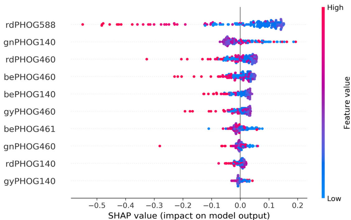
Fig. 5. Results of Shapley analysis performed on SVM (1 st order polynomial kernel) classifier.
