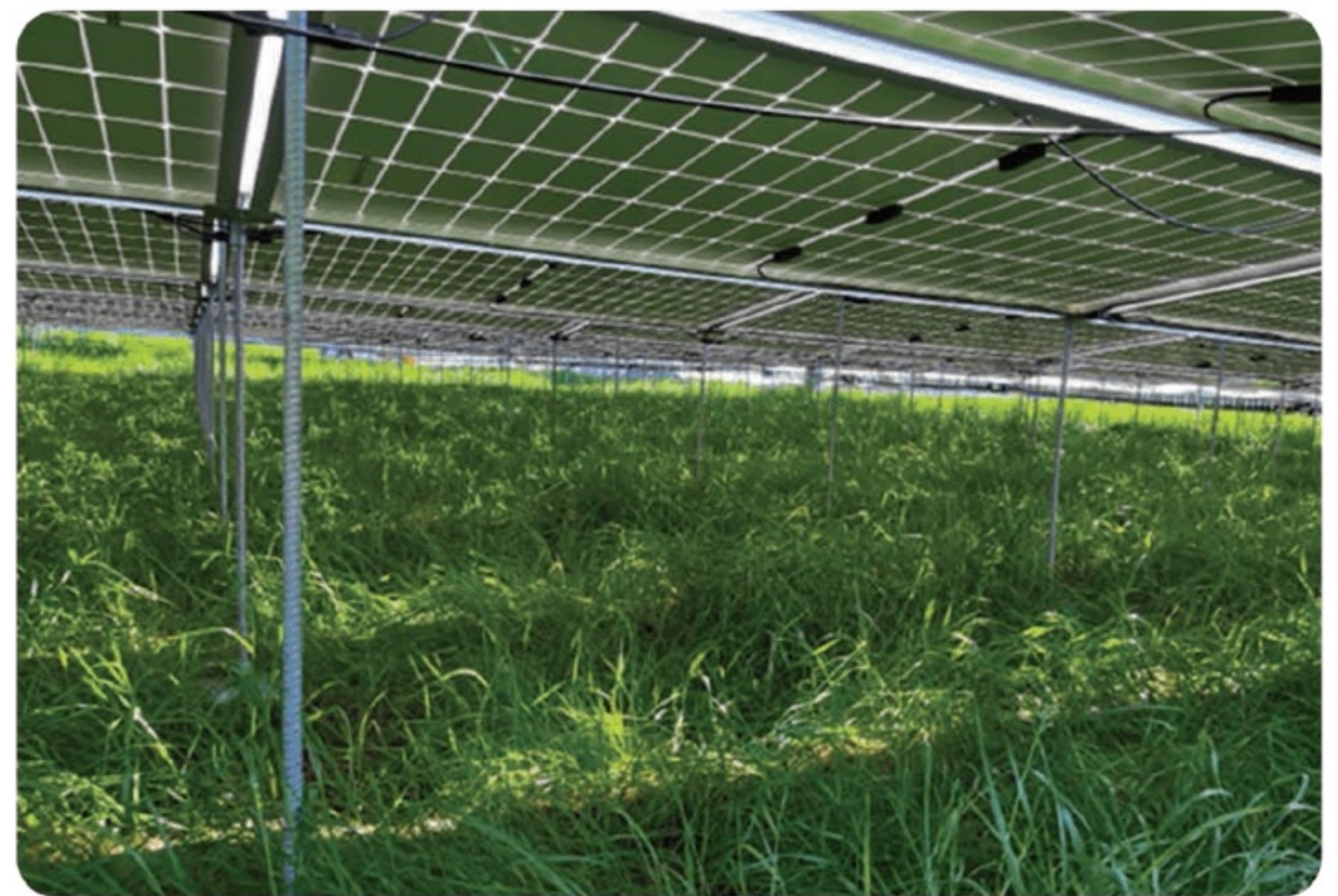
Vegetation (ryegrass) growing beneath a PEG array at the Junee Solar Farm
