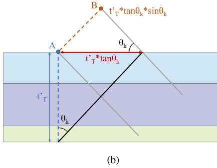
FIGURE 4. (a) Original locally non-planar structure and the equivalent thickness used to evaluate reflections in the discretized dome. (b) Effective locally-planar model that shows the phase compensation for the plane wave model.
