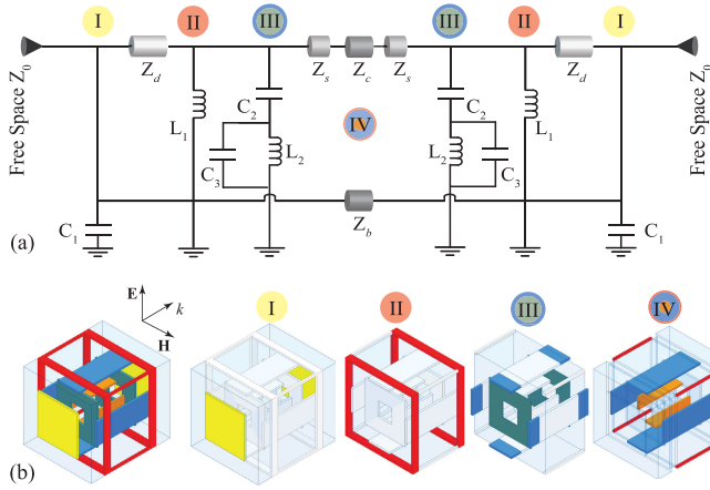
Fig. 12. Equivalent circuit-transmission line modeling for the dual-band 3-D meta-atom. (a) Lumped circuit elements C_1 = 12.95 fF, C_2 = 18.71 fF, C_3 = 16.83 fF, L_1 = 939.44 pH, and L_2 = 867.74 pH. The dielectric permittivities of the effective media are \epsilon_s = 1.28 , \epsilon_c = 0.24 , and \epsilon_b = 0.37 . (b) From the outermost (I) to the central (IV) divisions of the meta-atom. The electrical lengths of transmission lines are approximately \Theta_d = 29^\circ , \Theta_s = 27^\circ , \Theta_c = 114^\circ , and \Theta_b = 92^\circ when referenced at 30 GHz.
