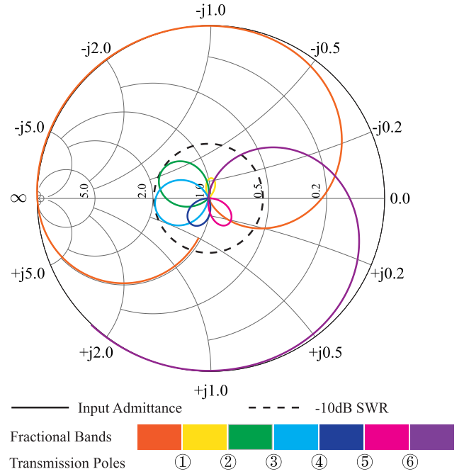
Fig. 10. Admittance Smith Chart for the revised 3-D meta-atom. The five knot-like loops correspond to the fractional bands in-between the six transmission poles. The rapid approach to and departure from the center of the locus indicates steep roll-off skirts at both the lowest and highest operating frequencies.
