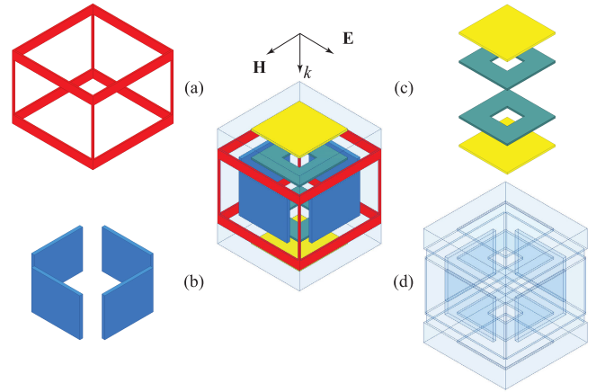
Fig. 1. Exploded view and assembly of the 3-D meta-atom evolved based on a 2-D centrally loaded prototype. (a)–(c) Conductive structures, including a hexahedral grid frame (red), side enclosures (blue), and a stack of square patches (yellow) and square rings (cyan), respectively. (d) Supporting dielectric.
