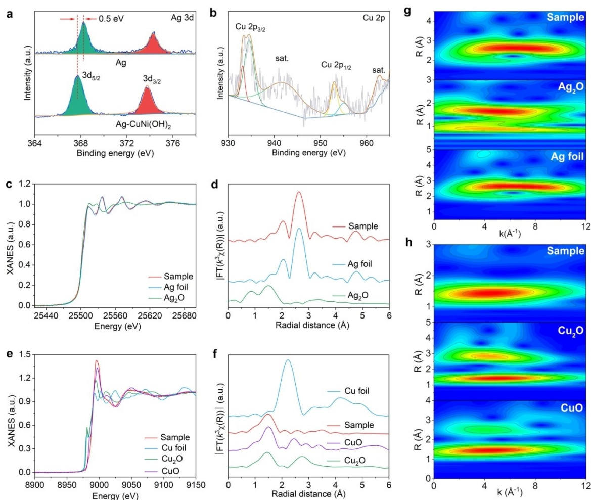
Figure 2. (a) Ag 3d and (b) Cu 2p spectra of Ag–CuNi(OH) 2 composite sample. (c) Normalized Ag K-edge XANES spectra of Ag–CuNi(OH) 2 sample with Ag foil and Ag 2 O reference samples, (d) k^3 -weighted Fourier-transform Ag K-edge. (e) Normalized Cu K-edge XANES spectra of Ag–CuNi(OH) 2 sample with Cu foil, Cu 2 O and CuO references, (f) k^3 -weighted Fourier-transform Cu K-edge. (g, h) Wavelet transforms of the k^2 -weighted Ag and Cu K-edge EXAFS signals for the high-coordination shells with Ag foil, Ag 2 O, Cu 2 O, and CuO as reference samples.
