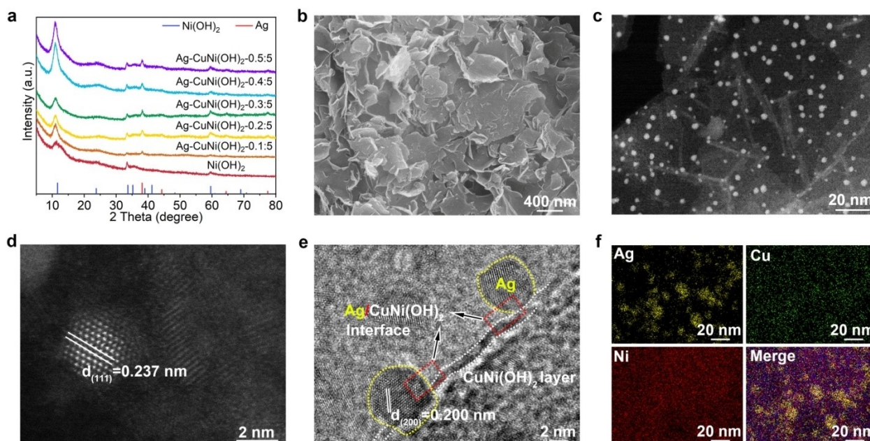
Figure 1. (a) XRD patterns of \text{Ag-CuNi}(\text{OH})_2\text{-}x with different Cu:Ag ratios ( x=0:5, 0.1:5, 0.2:5, 0.3:5, 0.4:5, \text{ and } 0.5:5 ). (b) Scanning electron microscope (SEM) image, (c,d) aberration-corrected high-angle annular dark-field scanning transmission electron microscope (HAADF-STEM) images, (e) high-resolution TEM (HRTEM) image and (f) elemental mapping images of \text{Ag-CuNi}(\text{OH})_2 sample (Ag, yellow; Cu, green; Ni, red).
