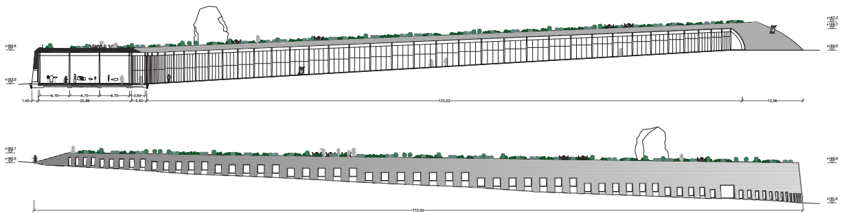
Museo Rapa Nui General plan, Cross Section and Elevation
