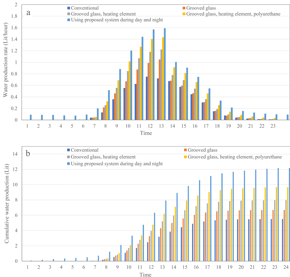
Fig. 5. Water production per hour per day (a) and cumulative water production per day (b) of proposed chess.
