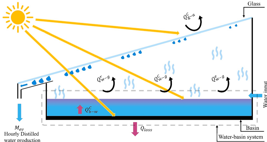
Fig. 2. Schematic diagram of the energy balance of the solar still single slope.
