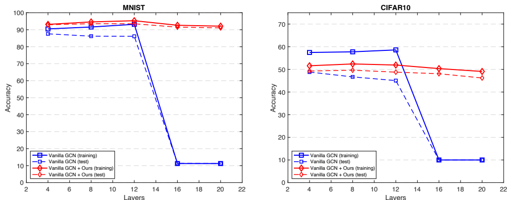
Figure 6: Performance of our method on the vanilla GCN with increased layers.
