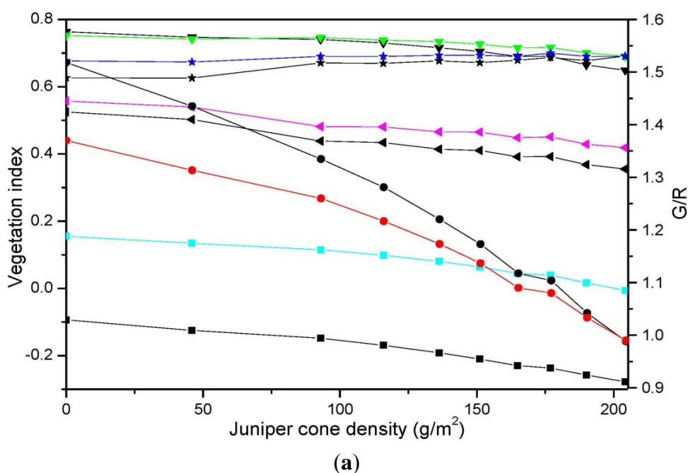
Figure 8. (a) Vegetation index and (b) Vegetation Index relative changeover different juniper cone densities, including MODIS broadband and narrow bands with the best-fit R^2 values in Table 2.
