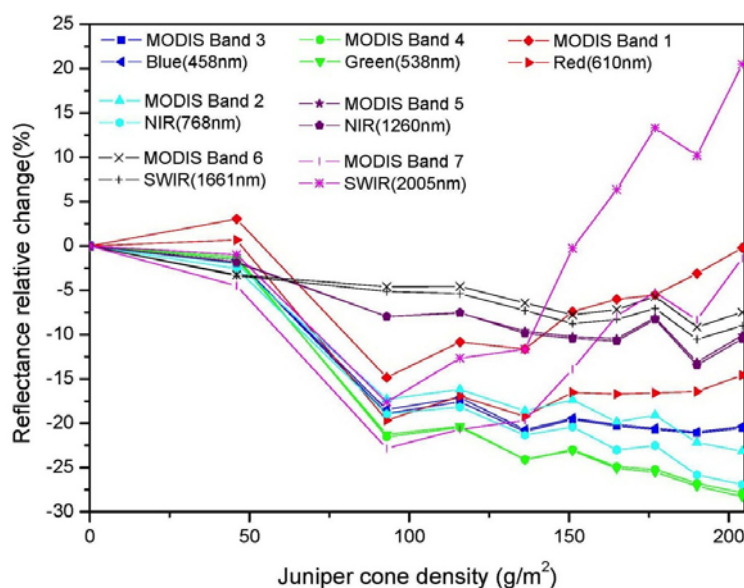
Figure 6. Relative changes in juniper canopy reflectance for different levels of juniper cone densities in MODIS Bands 1–7 and corresponding narrowband with the best-fit R^2 values.
