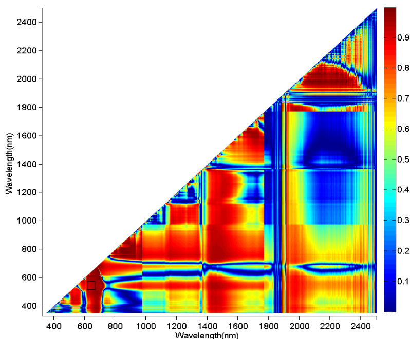
Figure 7. 2D correlation plots illustrating the coefficient of determination ( R^2 ) of linear regression between all possible Two-Band Vegetation Index (TBVI) and cone densities. The black square frame is the region of Green and Red corresponding to MODIS Bands 4 and 1.
