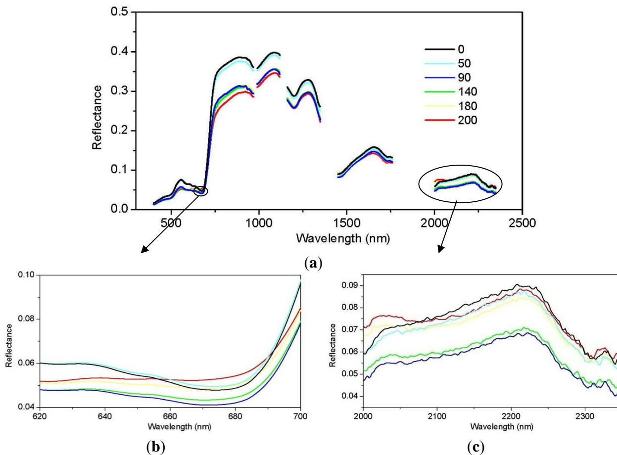
Figure 2. Juniper canopy spectral reflectance curves for variable cone densities (0, 50, 90, 140, 180, 200 g/m 2 ). Only six of the cone density levels are shown in order to more clearly depict the reflectance signature shifts.
