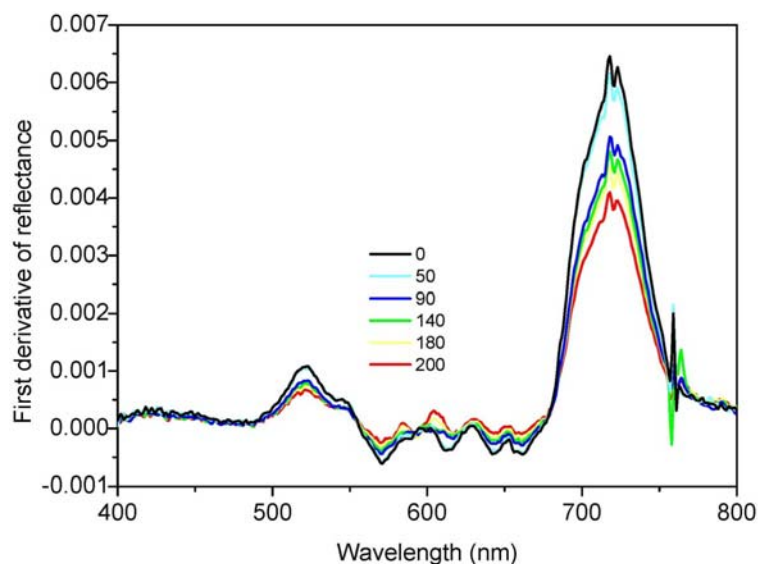
Figure 4. First derivative reflectance spectra across the visible and Near Infrared (NIR) region for the juniper canopy with varying cone density levels.
