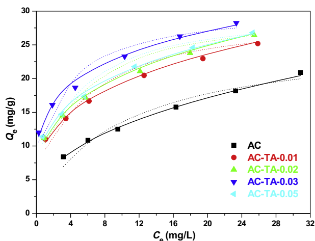
Fig. 1. Sorption isotherm of Cr(VI) on AC and AC-TA (dosage = 40 mg/50 mL; initial pH = 5.00 \pm 0.02 ; t = 48 h; and temperature = 22 \pm 1 °C).
