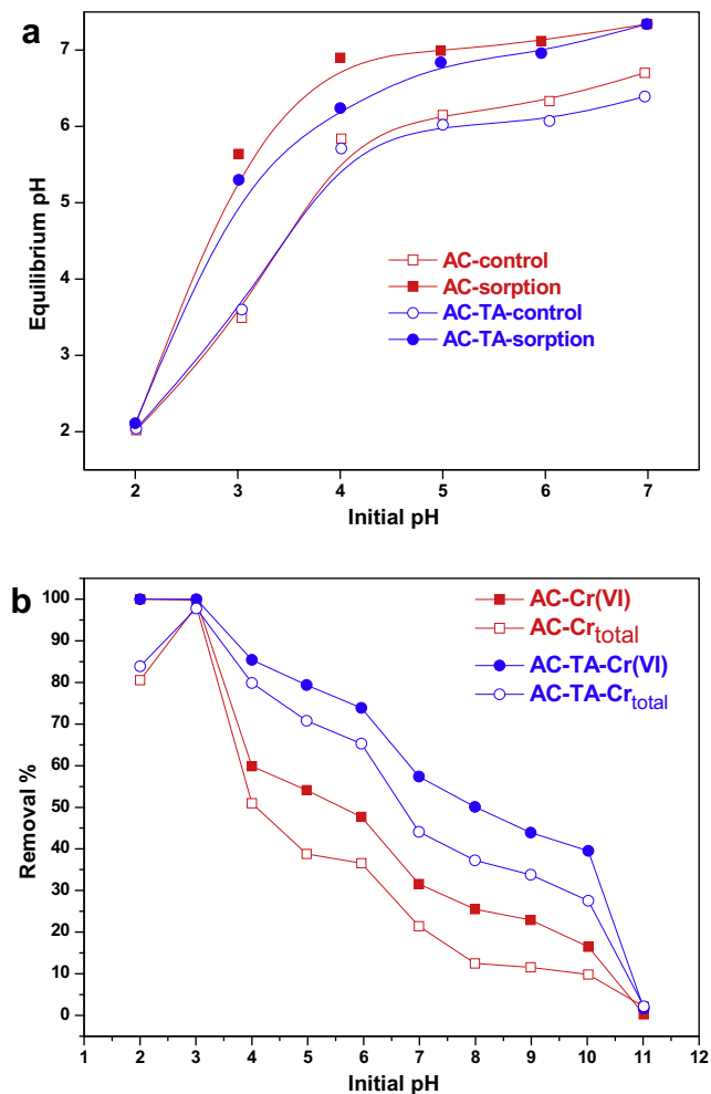
Fig. 2. Effect of initial pH on equilibrium pH in the present of or in the absence of Cr(VI) (a) and Cr removal on the carbons (b) (dosage = 40 mg/50 mL; C_0 = 20 mg/L; t = 48 h; and temperature = 22 ± 1 °C).
