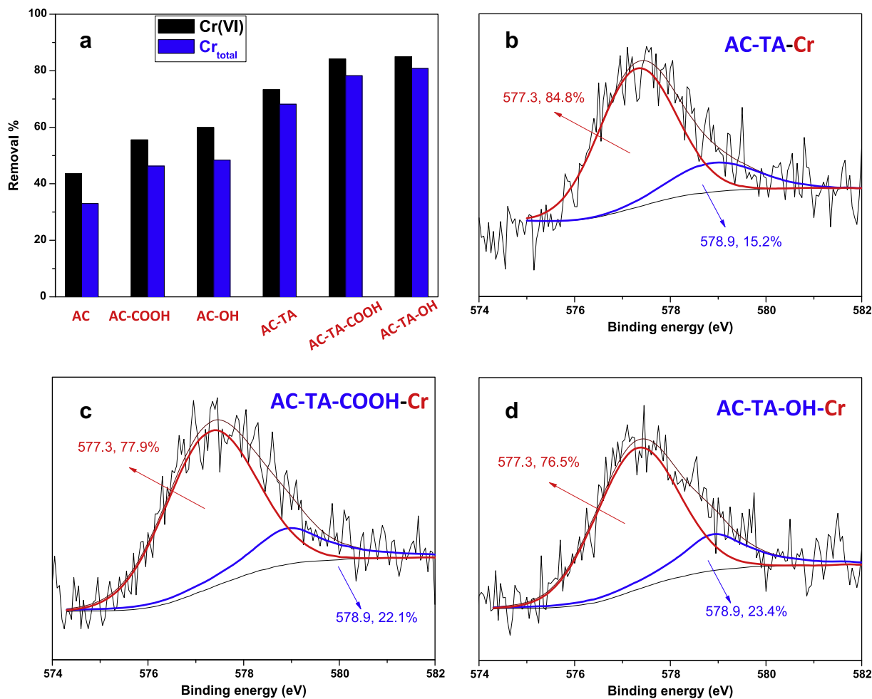
Fig. 6. Removal of Cr(VI) and Cr_{total} by AC and AC-TA before and after blocking of carboxyl and hydroxyl functional groups (a) (dosage = 40 mg/50 mL; C_0 = 20 mg/L; initial pH = 5.00 \pm 0.02 ; t = 48 h; and temperature = 22 \pm 1 °C). Cr 2p 3/2 XPS spectra of original AC-TA (b), AC-TA-COOH (c) and AC-TA-OH (d) after Cr(VI) sorption.
