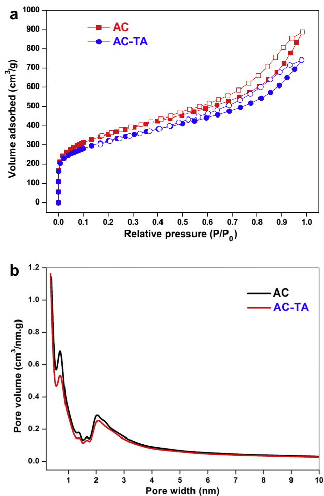
Fig. 3. N 2 adsorption/desorption isotherms (a) and pore size distribution (b) of AC and AC-TA.
