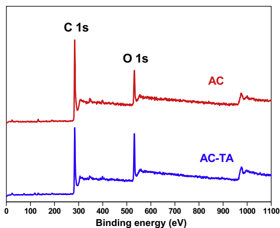
Fig. 4. XPS survey scans of AC and AC-TA.
