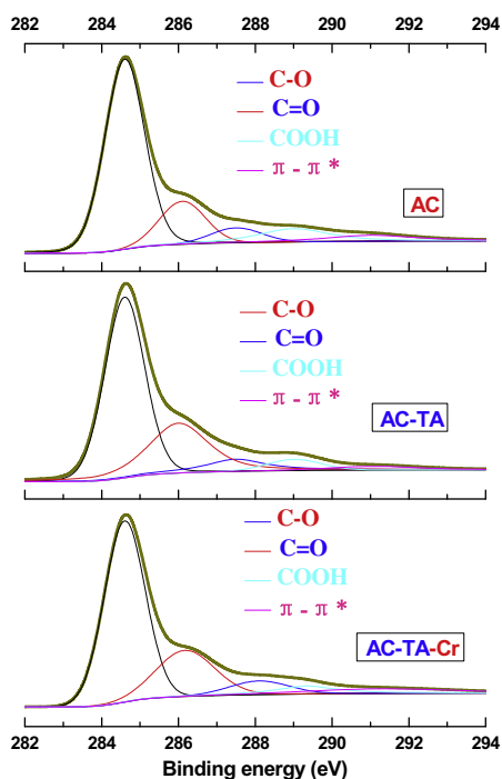
Fig. 5. High-resolution XPS spectra of C 1s for the carbons before and after Cr(VI) sorption.
