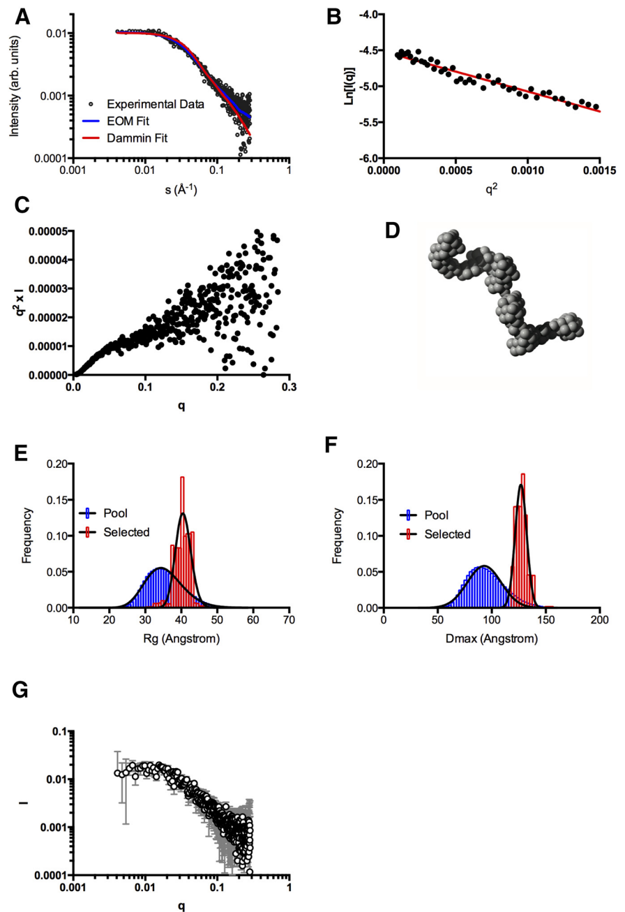
Figure 3. SAXS analysis of the A \beta /CQ complex. A , SAXS data for A \beta 1–42 (0.2 mg/ml, \sim 20 \mu\text{M} ) in the presence of 20 \mu\text{M} CQ was acquired at the Australian synchrotron. B , Guinier analysis of the CQ data in A . C , Kratky analysis of the CQ data in A . D , De novo reconstruction of the scattering entity induced by CQ using Dammin. Line indicates overall dimension ( D_{\text{max}} ). E , F , Ensemble optimization modeling of the CQ-induced A \beta 1–42 dimers provides information on the distribution in the radius of gyration ( R_g , E ) and maximal dimension ( D_{\text{max}} , F ) in relation to a pool of randomly generated structures: blue represents pool; red represents selected structure parameters. G , SAXS data for A \beta 1–42 (0.2 mg/ml, \sim 20 \mu\text{M} ) in the presence of 20 \mu\text{M} PBT2 (red squares) were also acquired at the Australian synchrotron but had too high a ratio of signal-to-noise and thus were not of sufficient quality for further analysis.
