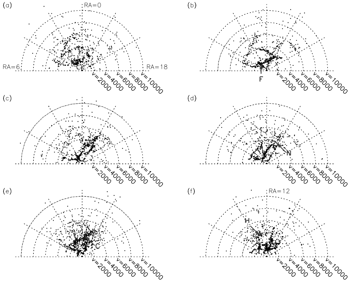
Figure 13. Velocity distribution of HICAT sources divided into segments all hinged on the equatorial plane at the 6–18 h line starting with segment (a) with one side lying in that plane centred at R.A. = 0 h, (b) above that and so on, with (f) again with one side in the plane, but centred at R.A. = 12 h.
