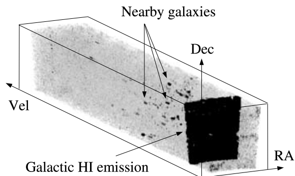
Figure 1. Orthogonal projection of HIPASS cube 93 showing emission from the Milky Way as well as other nearby galaxies. Velocity range is truncated at 10\,000 \text{ km s}^{-1} .
