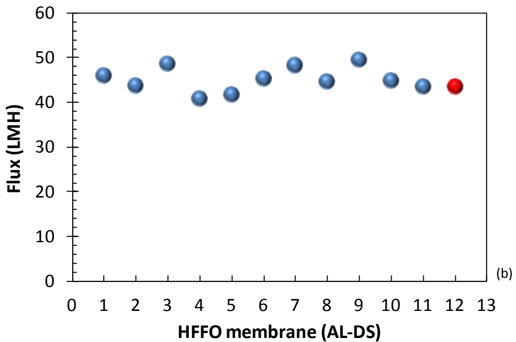
Fig. 6. Performances of FO membrane after cleaning a) resultant flux for membrane used at AL-FS orientation b) resultant flux for membrane at AL-DS orientation. Red circle shows the baseline flux.
