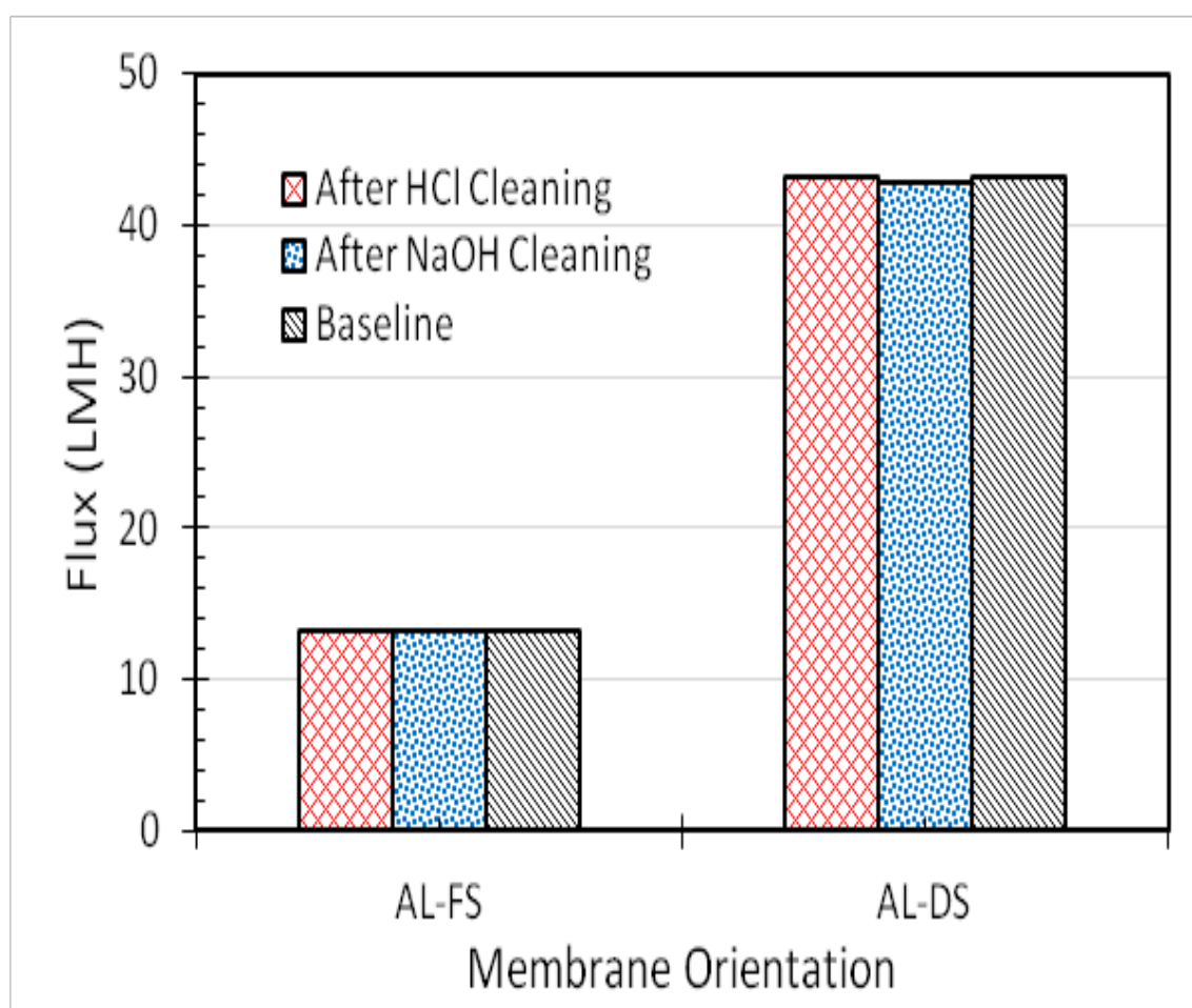
Fig. 4. Performances of HFFO membrane chemical cleaning using HCl and NaOH. BGW35 FS was used in fouling experiments.
