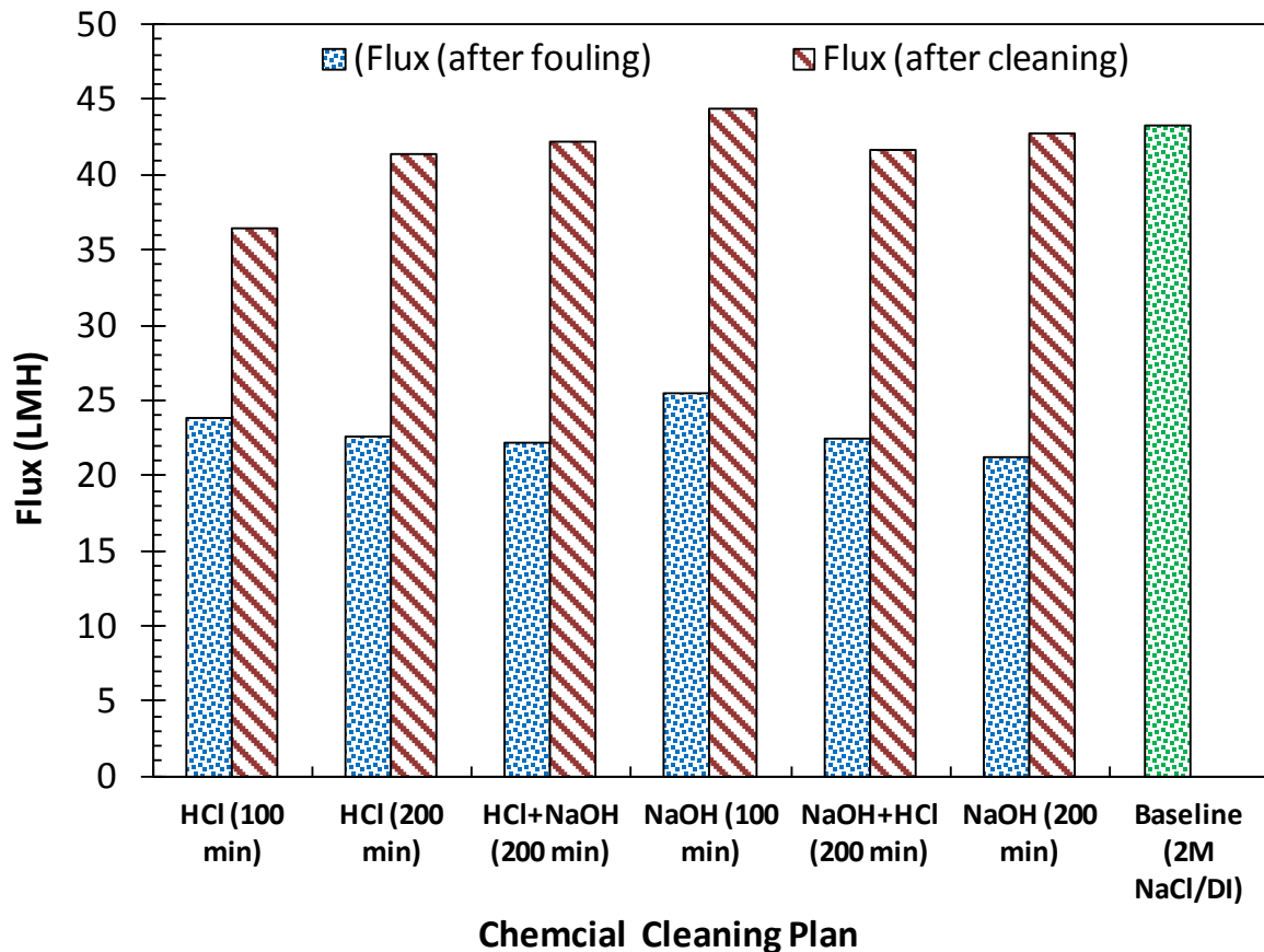
Fig. 5. Performances of various combinations of chemicals (HCl and NaOH) for HFFO membrane cleaning. Membrane was used for fouling experiments in AL-DS orientation.
