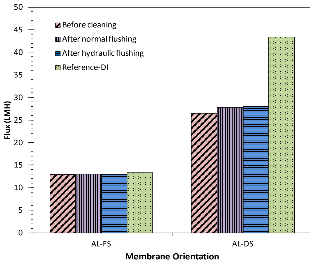
Fig. 3. Effect of physical cleaning of HFFO membrane for AL-FS and AL-DS orientation. 2 M KCl DS and 60 mg/L each of HA and BSA were used with BGW35 quality FS for the fouling test. Normal flushing was carried out at crossflow rates representing Re of 1900 and 700 whereas fast hydraulic flux used higher crossflow Re. of 2350 and 1450 for lumen side
