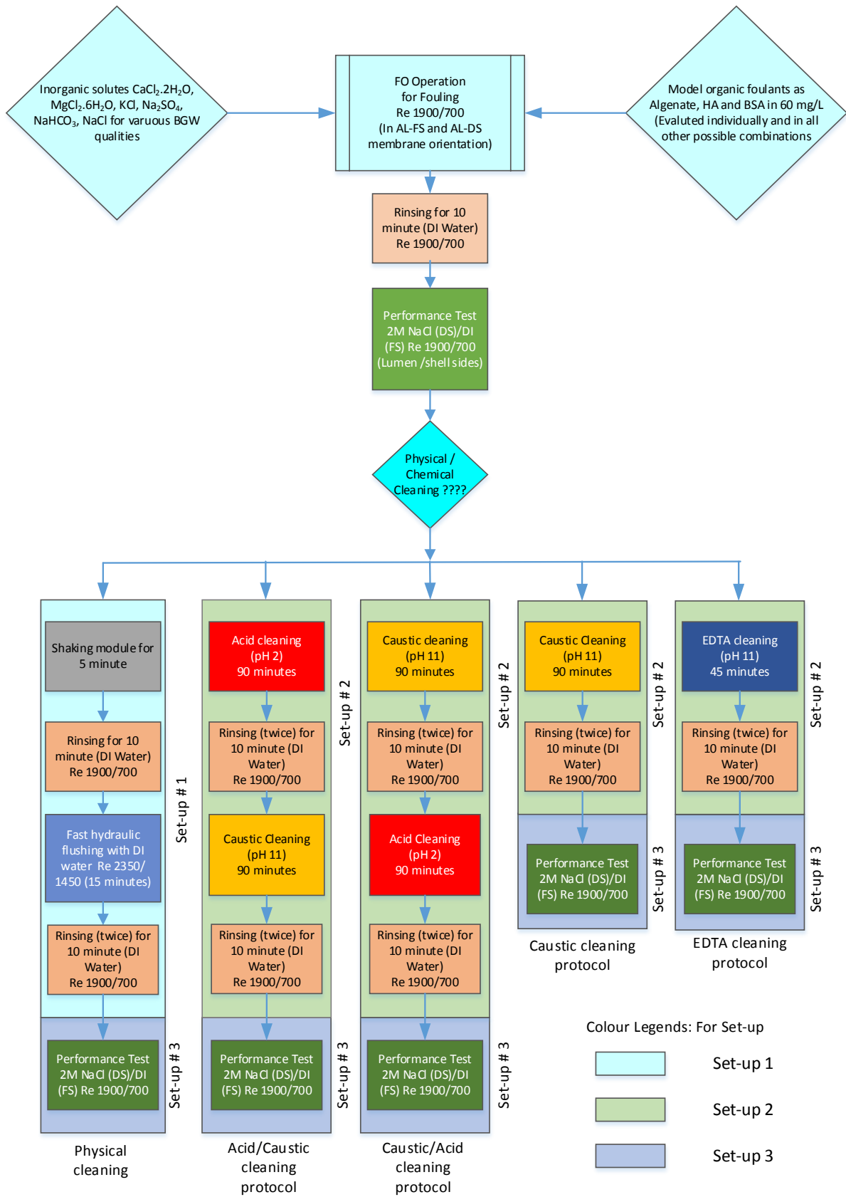
Fig. 1. Sequence of different physical and chemical membrane cleaning procedures used for this study
