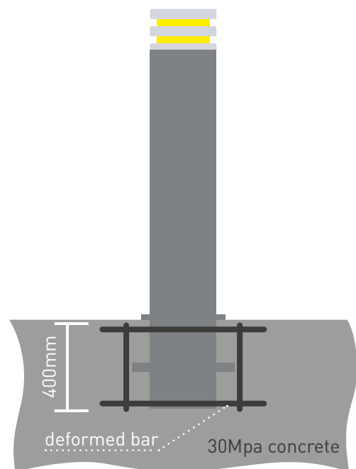
FOUNDATION REQUIREMENTS
