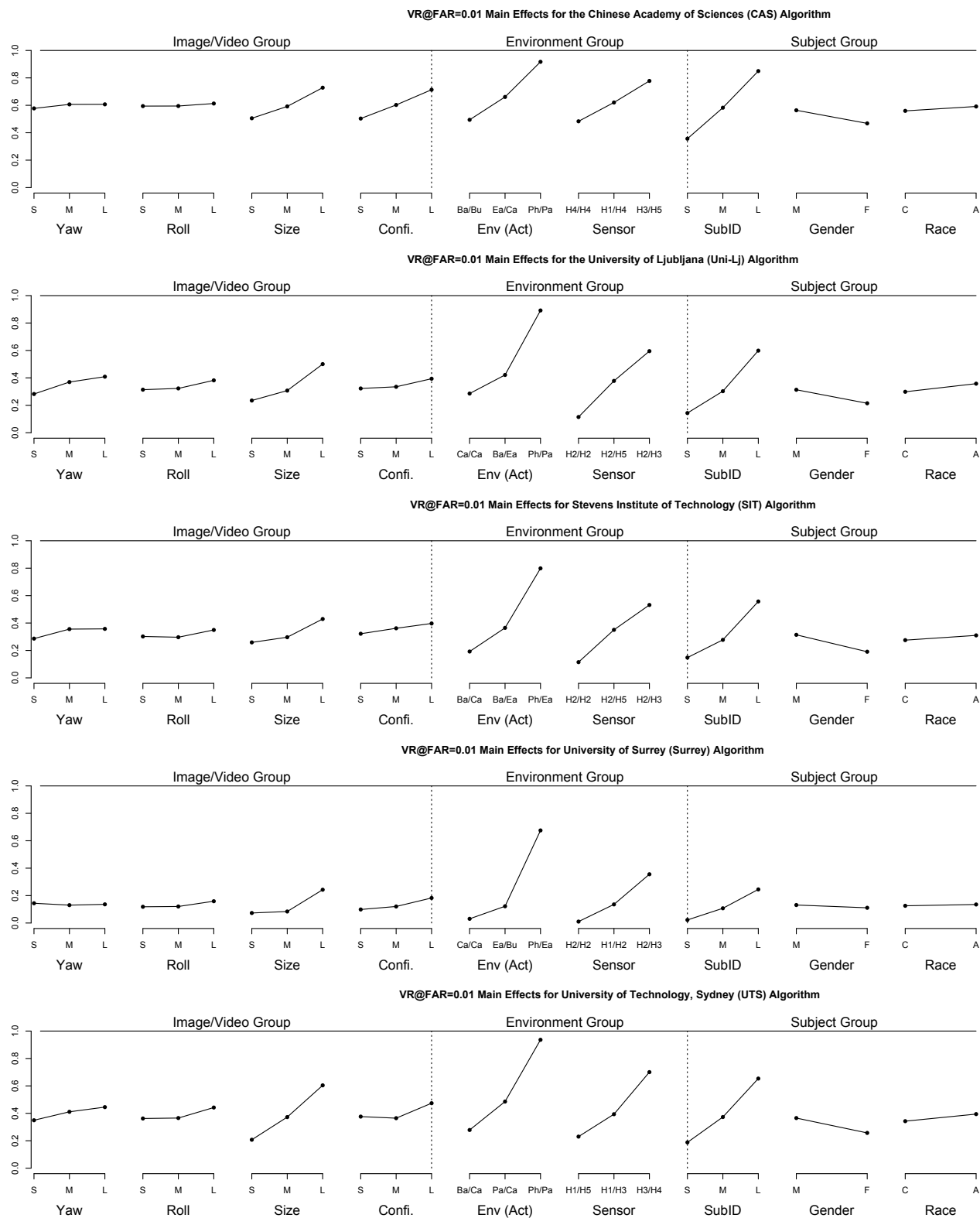
Fig. 3. Marginal analysis of verification rate change conditioned on different factors.
