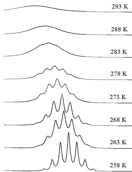
Fig. 7 Selected portion of the 600 MHz 1 H spectra for Na(dipdte) \cdot 5H 2 O in CD 3 CN, showing the change in H2 resonance as a function of temperature.
