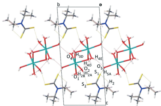
Fig. 3 Molecular packing diagram as viewed along the a axis, showing layered morphology of Na(dipdctc)·5H 2 O.
