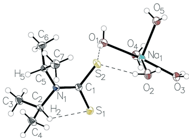
Fig. 2 The structure the Na(dipdte)·5H 2 O asymmetric unit showing the atom-labelling scheme and thermal displacement ellipsoids at 50% probability.
