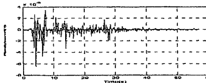
Fig. 10. Floor displacement using ASMC-2 MR dampers
