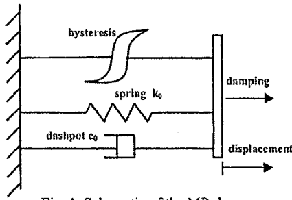
Fig. 1. Schematic of the MR damper
