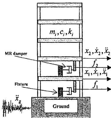
Fig. 4. The building model with 2 MR dampers
