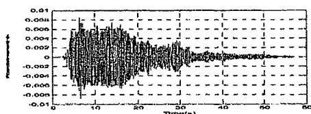
Fig. 6. Floor displacement-uncontrolled
