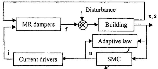
Fig. 3. Block diagram with adaptive sliding mode
