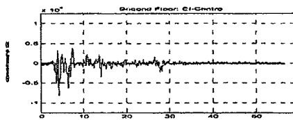
Fig. 12. Control force of MR damper at second-floor
