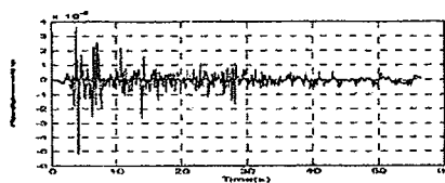
Fig. 9. Floor displacement using SMC-2 MR dampers
