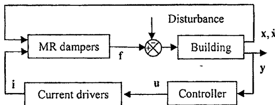
Fig. 2. Block diagram of the control system
