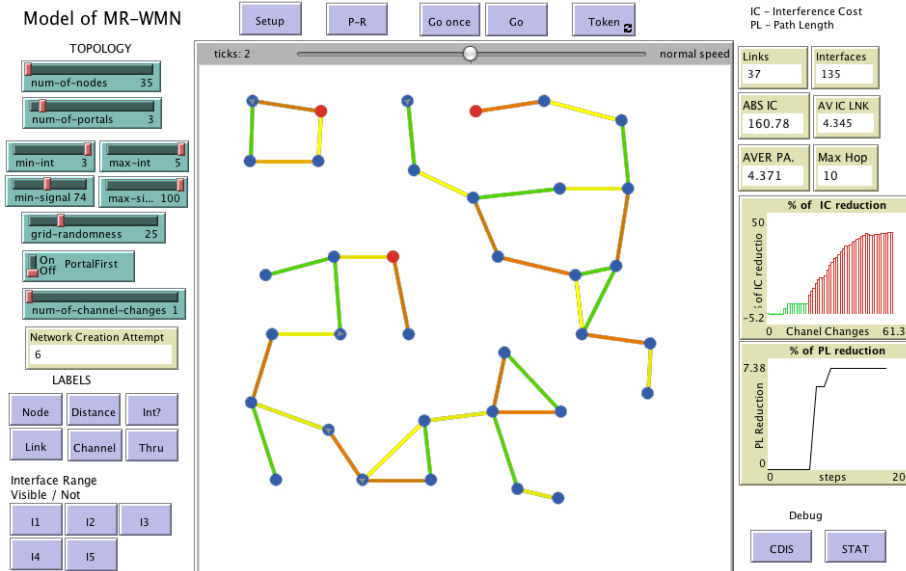
Fig. 1. The implementation of the algorithms.
